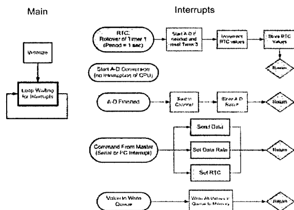
Figure 21. Top level flight software architecture
