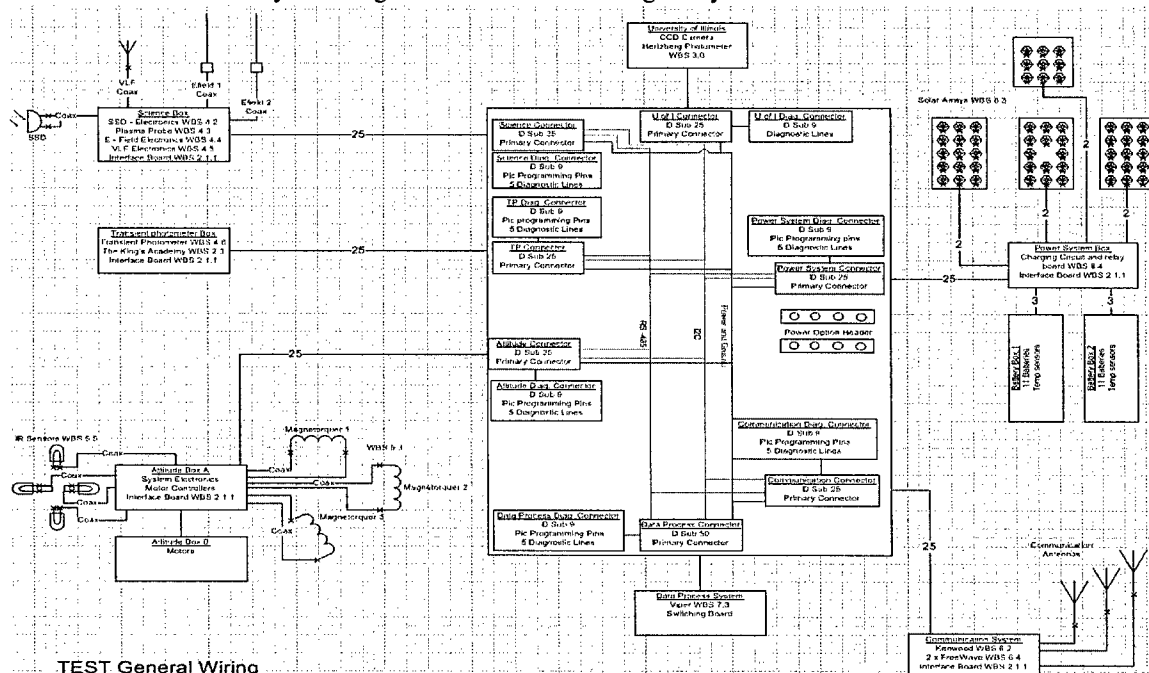
Figure 10. Wire Harness System
