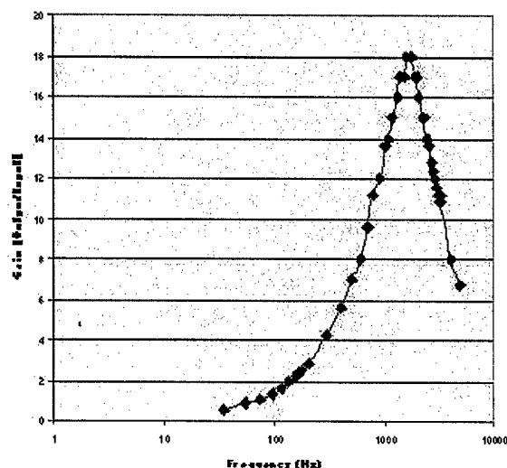
Figure 2b. VLF Frequency Response
