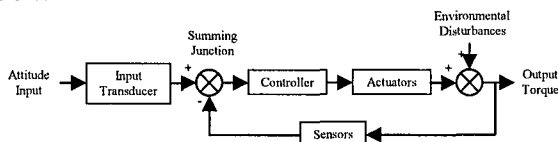
Figure 16. Basic Control Loop
