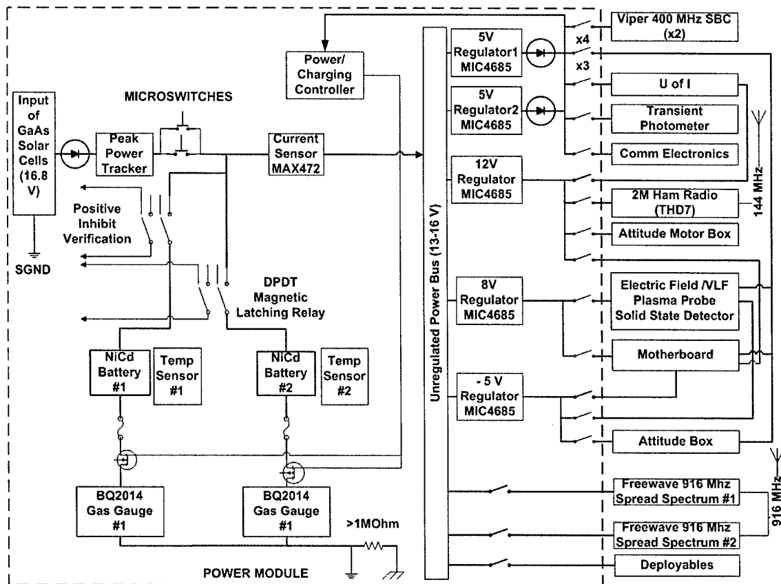
Figure 14. Power System Diagram
