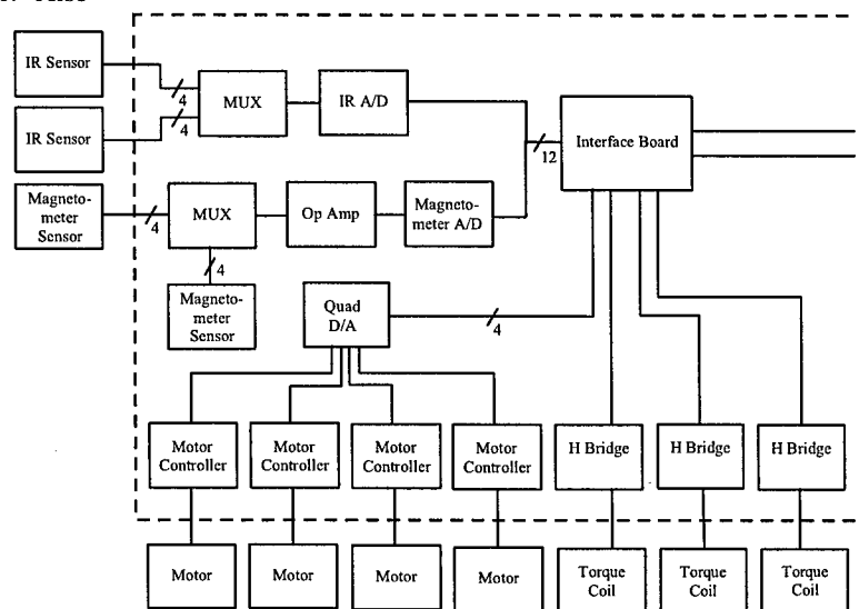
Figure 17. Attitude Electronics Control Module
