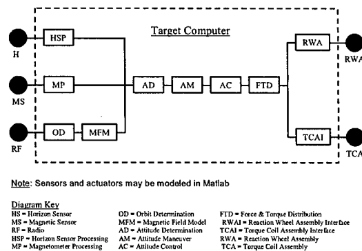
Figure 19. Top level flight software architecture
