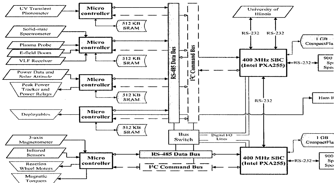
Figure 20. Processor system
