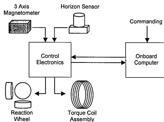
Figure 14. Attitude control system diagram
