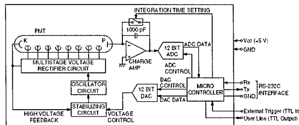
Figure 5. Logic Diagram of H7468.
