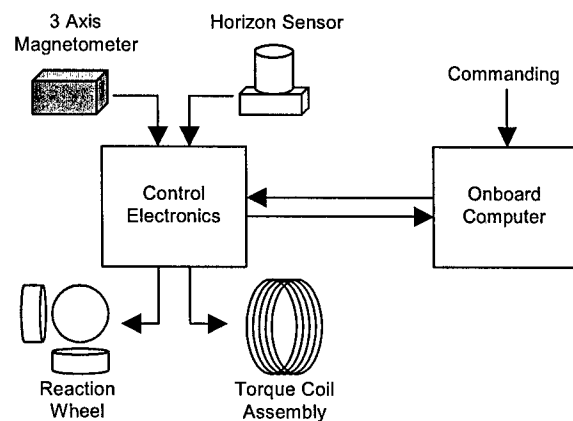
Figure 16. General Attitude System Diagram
