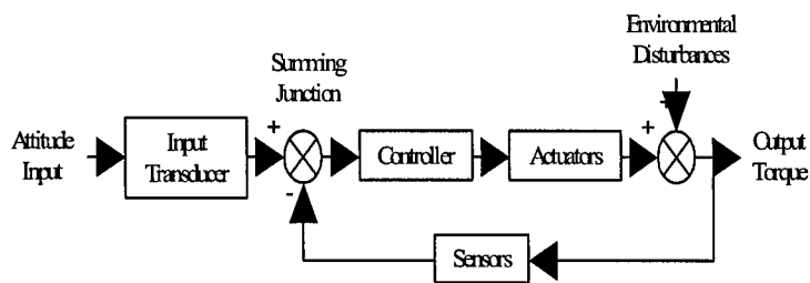
Figure 18. Basic Control Loop
