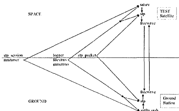
Figure 20. Software function calls
