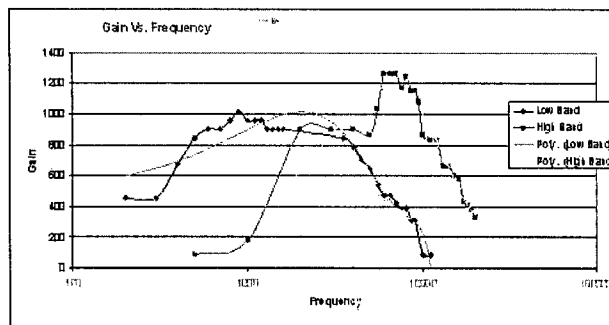
Figure 3. VLF Frequency Response
