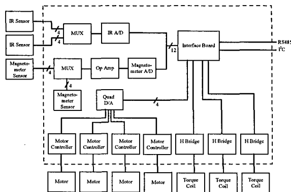
Figure 15. Attitude Control Electronics Module
