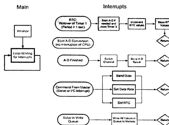
Figure 19. Software flow diagram
