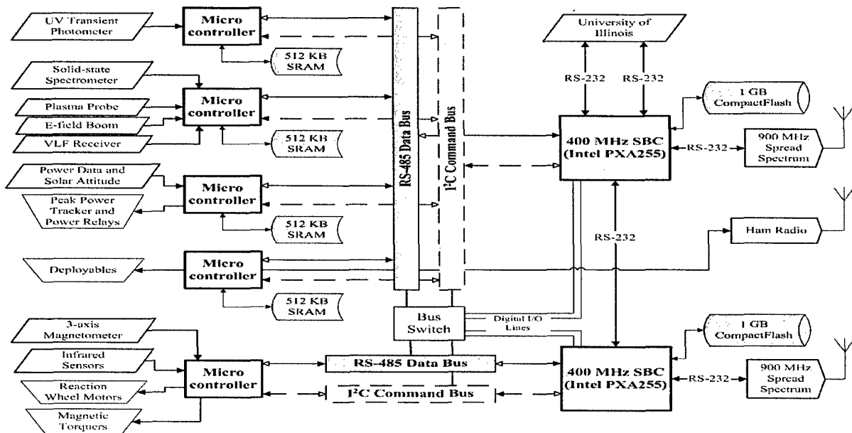
Figure 18. Processor system COMMAND AND DATA HANDLING
