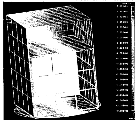
Figure 9. IDEAS modular thermal model
