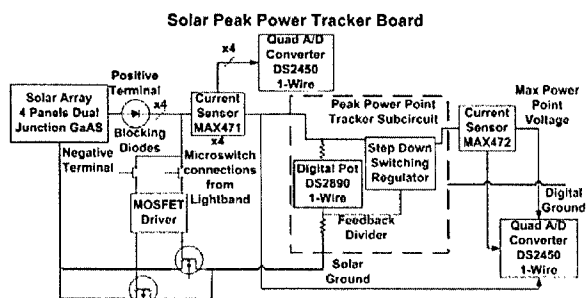
Figure 13. Solar peak power tracker board
