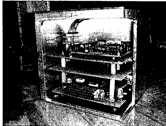
Figure 5. Cut away of module to show PCB stack
