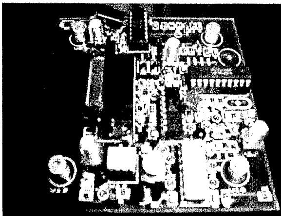
Figure 2a. Science Module Interface PCB
