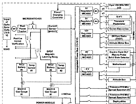
Figure 12. power system diagram
