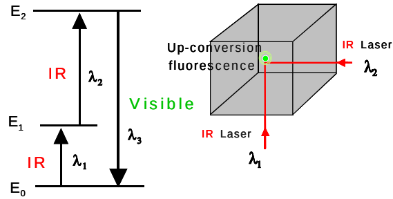
Figure 2: Schematic diagram of static volume 3D display. Two frequency two step process is shown on the left hand. Voxel is generated in the display medium by two different frequency IR laser beam at the cross point.
