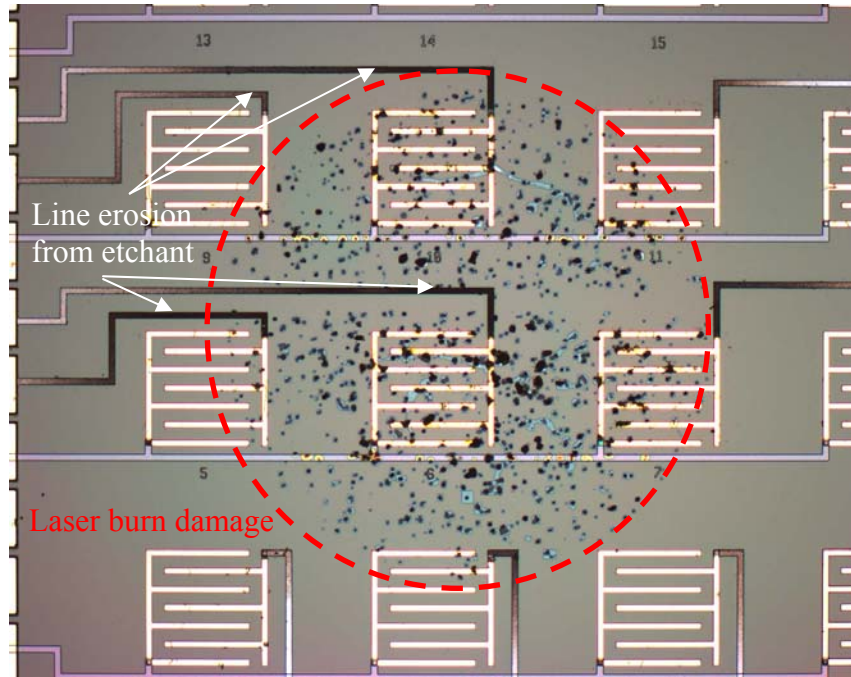
Figure 54. Front view of Suspended Membrane Pixel System with 1 mm diameter laser etch after wet chemical etch for 45 minutes in 12.5% KOH W/V at 85 °C.
