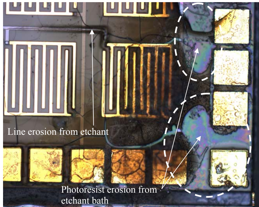
Figure 52. Suspended Membrane Pixel Sensor secured to glass slide using photoresist and exposed to etchant bath of 12.5% KOH W/V at 80 °C for 3 hours.
