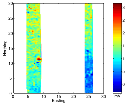
Figure 4.8: Gridded images of channel 1 EM63 data with medium repetition rate collected on part of Navy QA Grid 2E. The grid has been rotated and translated to local co-ordinates.
