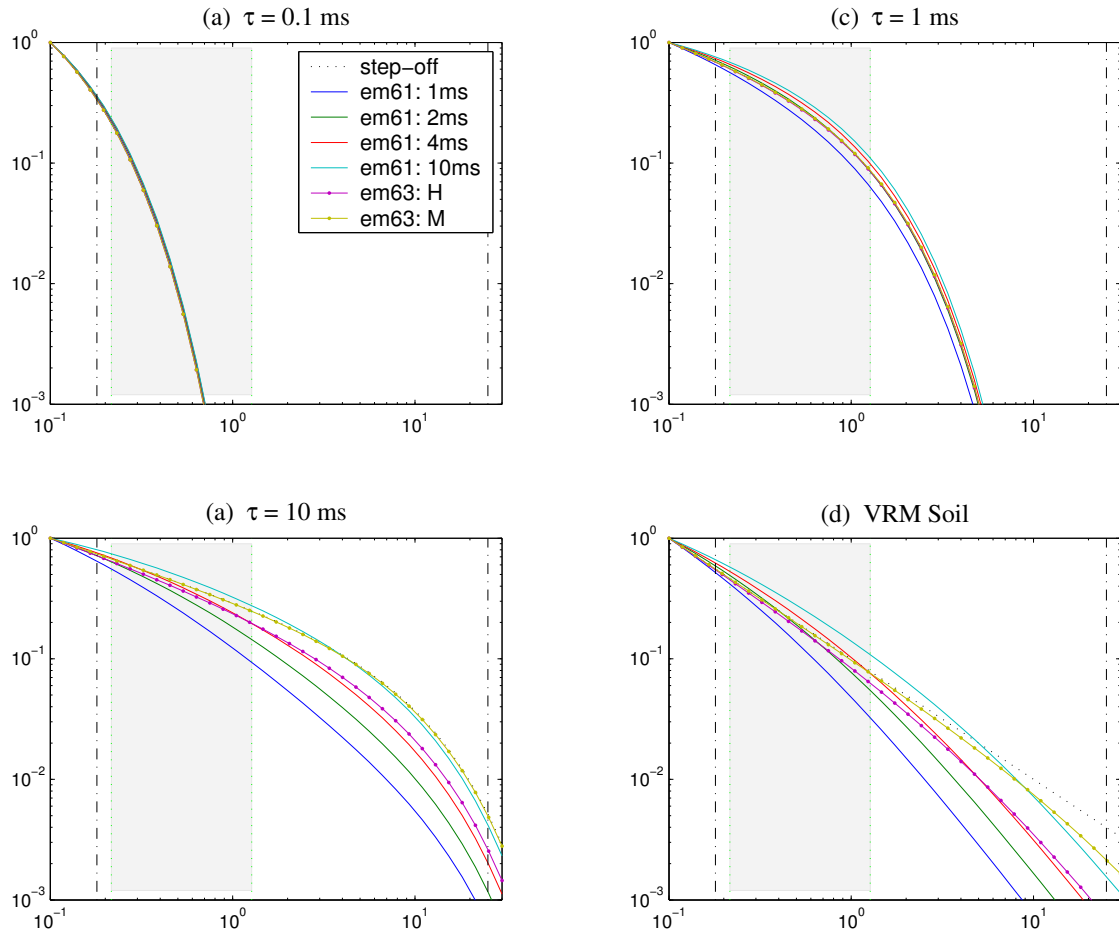
Figure 6.1: The effect of different waveforms on different time constant targets. The grey area represents the measurement range of the standard EM61Mk2 TEM sensor.
