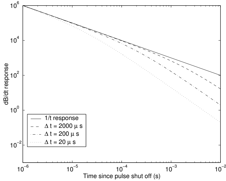
Figure 3.2: Effect of pulse length on the ferrite decay.
