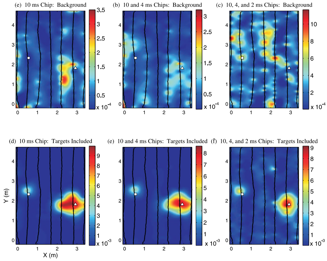
Figure 6.4: Misfit comparison.
