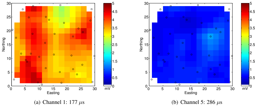
Figure 4.18: Gridded images of EM63 sounding data collected on the unseeded grid at the Waikoloa GPO. Panel a) Channel 1 and b) Channel 5. The data were collected with the medium repetition rate. The grid has been rotated and translated to local co-ordinates.
