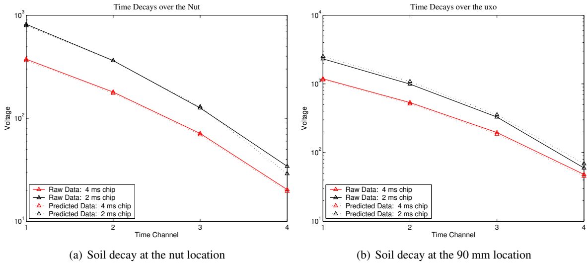
Figure 6.14: Decay comparisons.
