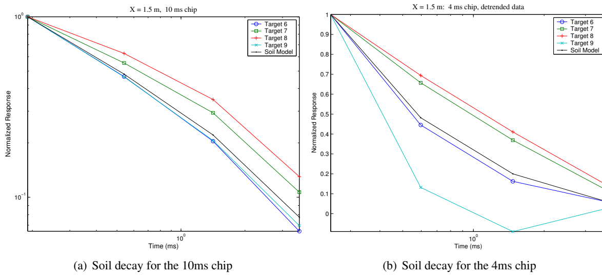
Figure 6.30: Decay comparisons.
