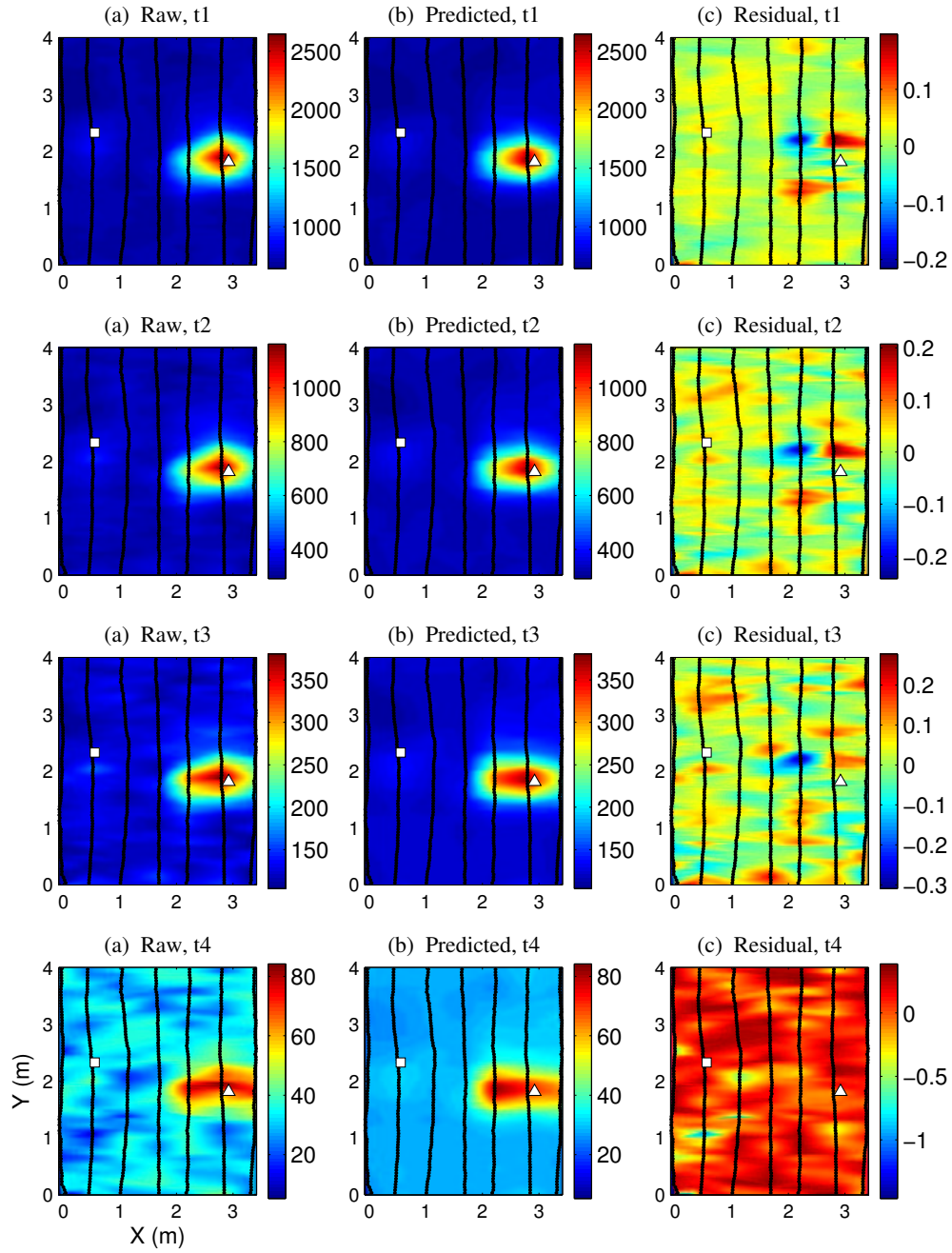
Figure 6.11: Comparison of 2ms chip raw data and the 2ms data predicted from the 10ms chip data. The bolt and UXO are present for this data.
