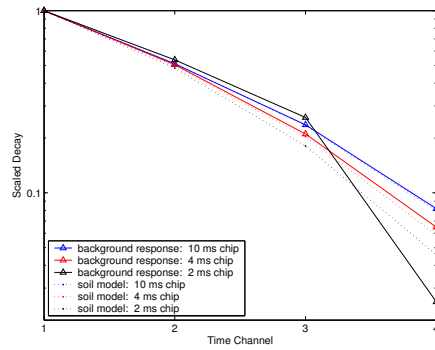
(a) Soil decay at the nut location
