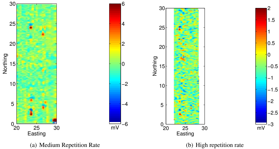
Figure 4.16: Gridded images of channel 1 EM63 data collected on a section of the Waimea seeded grid using two different repetition rates. Panel a) medium repetition rate and b) high repetition rate. The grid has been rotated and translated to local co-ordinates.
