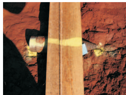
(b) Photo of 90 mm UXO
