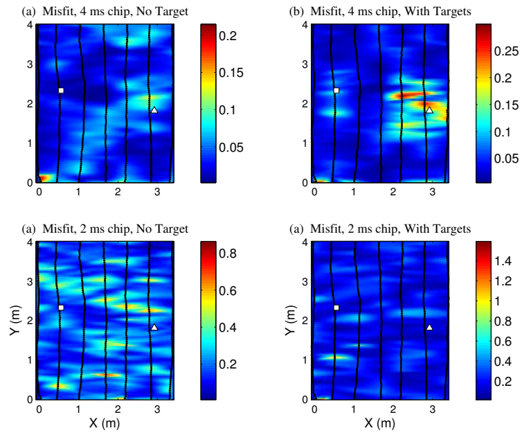
Figure 6.15: Comparison of misfits when applying the differential.
