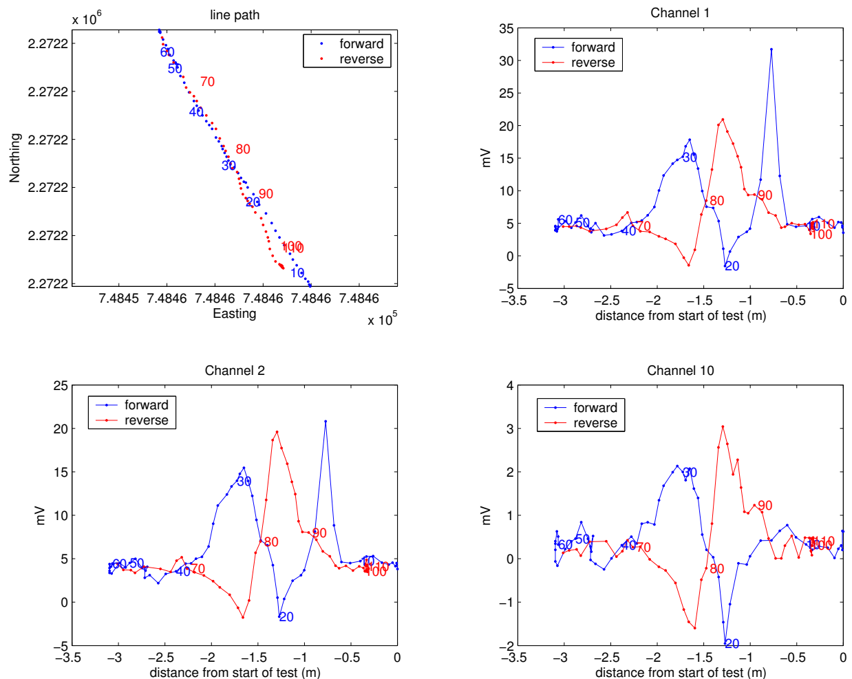
Figure 4.7: Lag test from Sept 28, 2004. EM63 data collected using the medium repetition rate.
