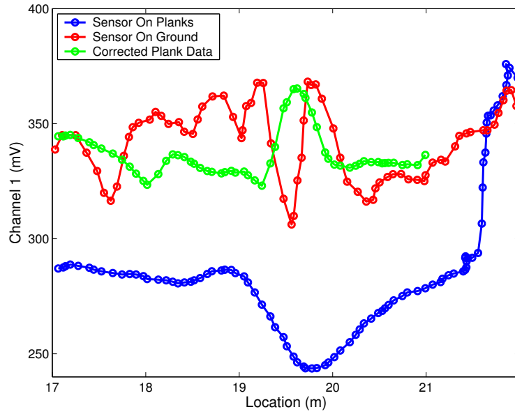
Figure 5.6: Data collected along Line 2 of the plank grid (shown as a magenta dashed line in Figure 5.1). The blue line with circles is the data collected on the planks, red line with circles is the data collected on the ground and the green line with circles is the height corrected plank data. The rivulet is located at approximately 19.8m N and the end of the planks is located at approximately 21.5m N.
