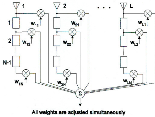
Figure 1. A block diagram of STAP based adaptive arrays, Delay between taps = T_0 .
