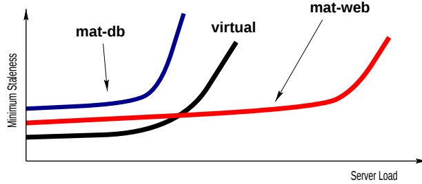
Figure 5: Minimum staleness under heavy loads
