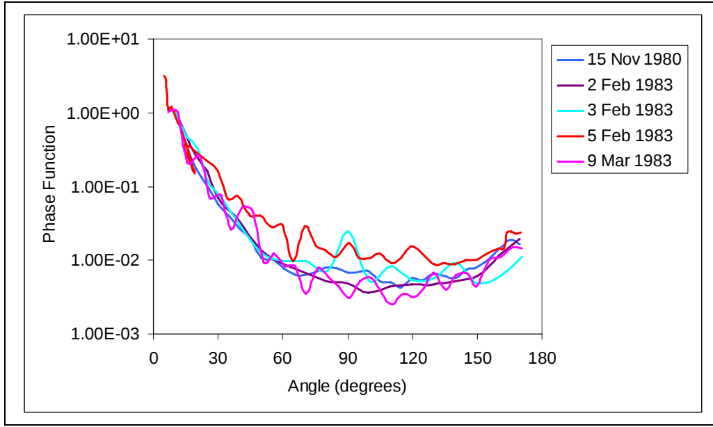
Figure 4. Snow phase function measurements taken by Winchester at 0.6238 \mu\text{m} .
