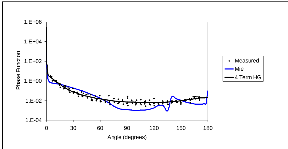
Figure 5. Phase function comparison of the 4-term HG (solid black) with the Mie (solid blue) at 0.6238 \mu\text{m} . Winchester's measurements are represented by the solid diamond shaped symbol (black).
