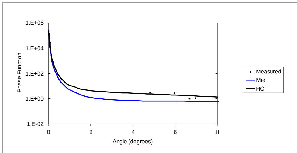
Figure 6. Peak phase function comparison ( 0^\circ to 8^\circ ) of the 4-term HG (solid black) with the Mie (solid blue) at 0.6238 \mu\text{m} . Winchester's measurements are represented by the solid diamond shaped symbol (black).
