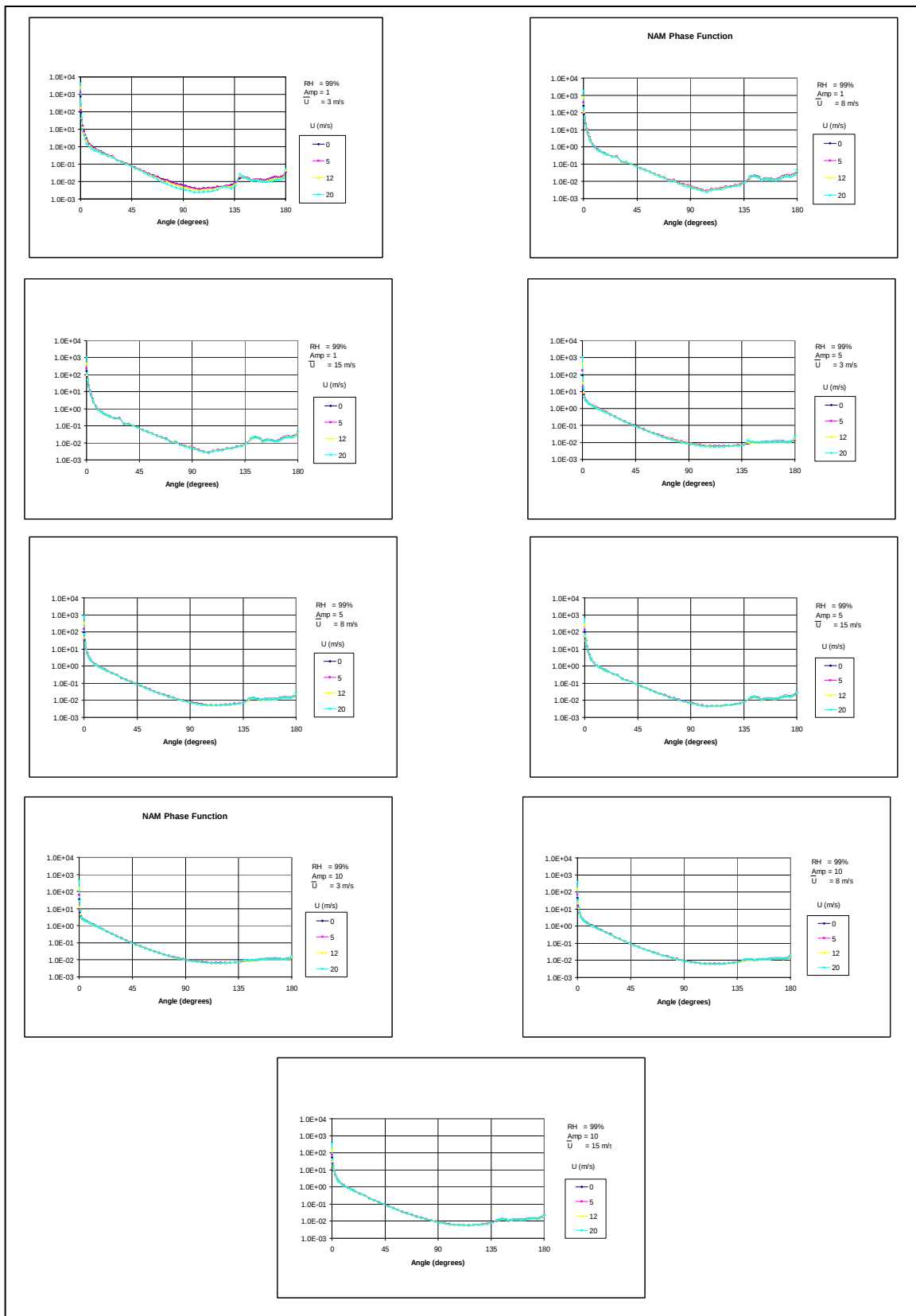
Figure 1. NAM phase functions at 0.55\mu\text{m} and 99% RH as a function of AMP, current ( U ), and average ( \bar{U} ) wind speed.
