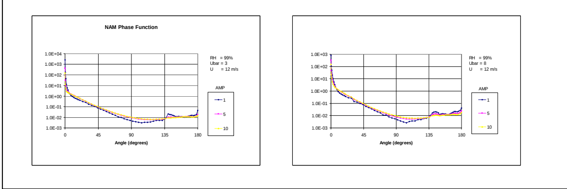
Figure 3. NAM phase functions at 0.55\mu\text{m} , 99% RH, current wind speed ( U ) of 12 m/s, and average wind speeds ( \bar{U} ) of 3 and 8 m/s as a function of AMP.
