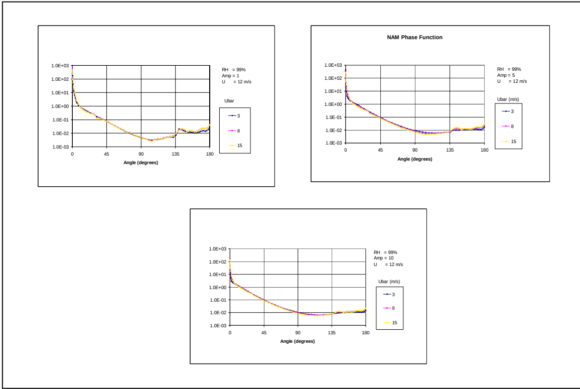
Figure 2. NAM phase functions at 0.55\mu\text{m} , 99% RH, current wind speed ( U ) of 12 m/s, and AMPs of 1, 5, and 10 as a function of the average wind speed \bar{U} .
