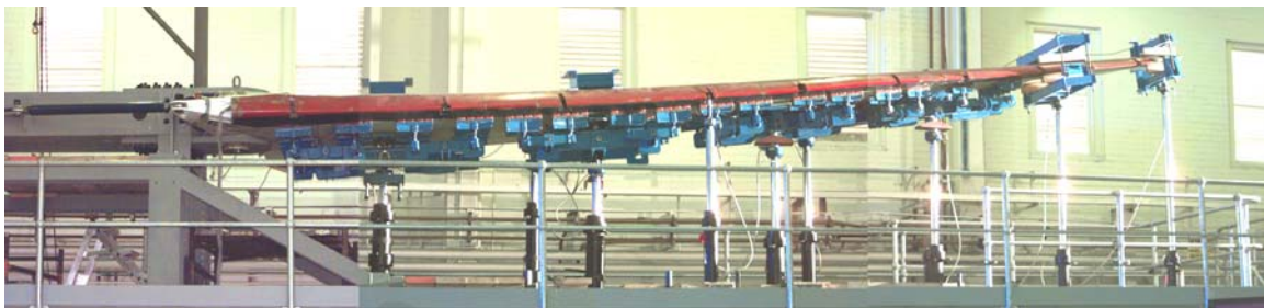
Figure 32: Wing A15-5 in the test rig at 50% of maximum positive proof load
