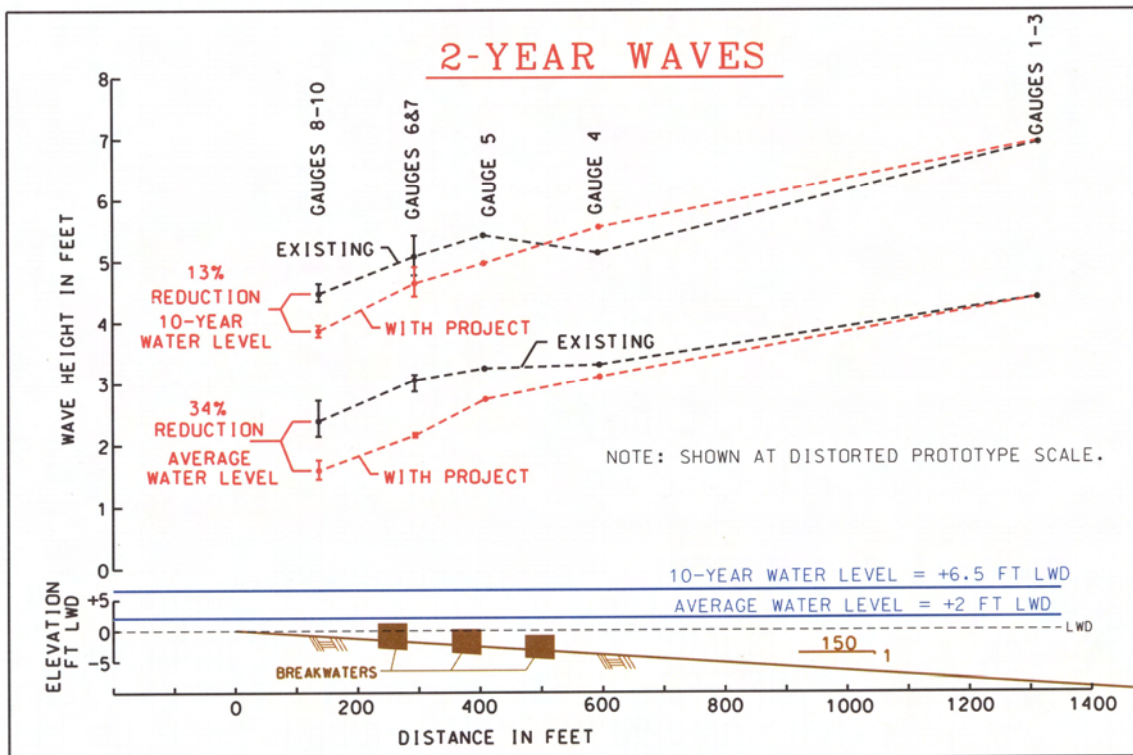
Figure 13. 2-year wave summary graph
