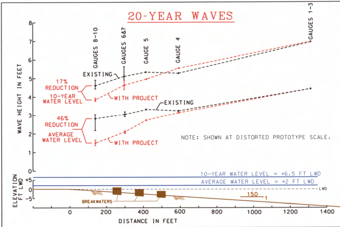
Figure 12. 20-year wave summary graph
