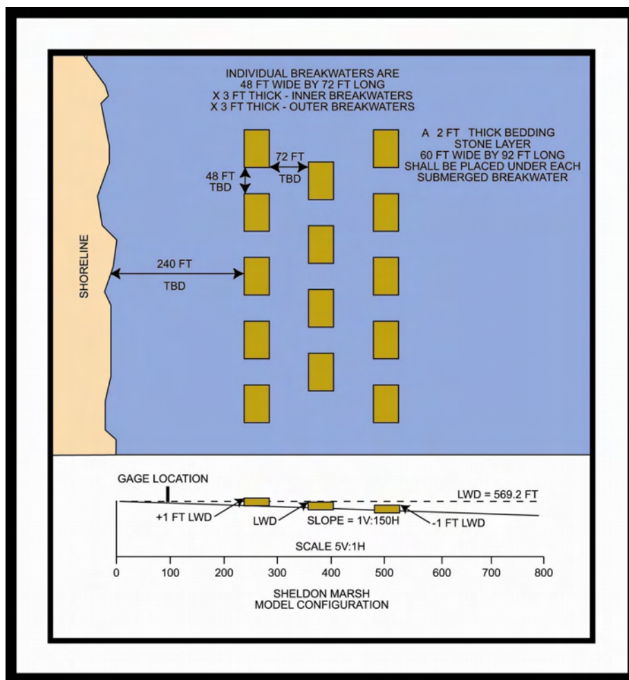
Figure 11. Model configuration with real-world dimensions
