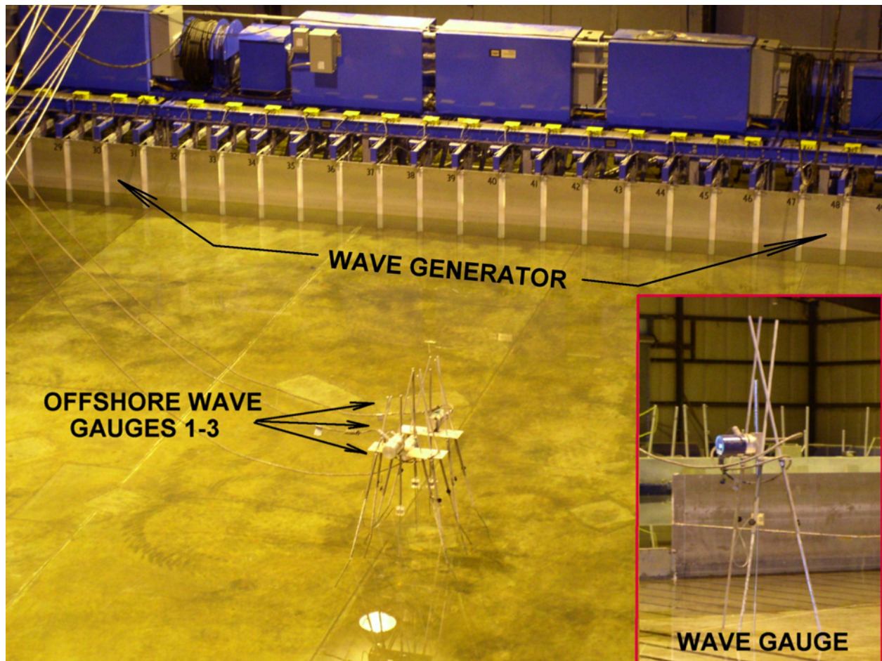
Figure 8. Photograph of wave generator and gauge configuration
