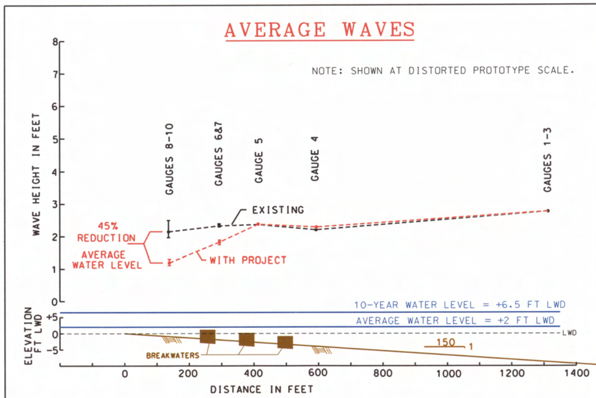
Figure 14. Average wave summary graph
