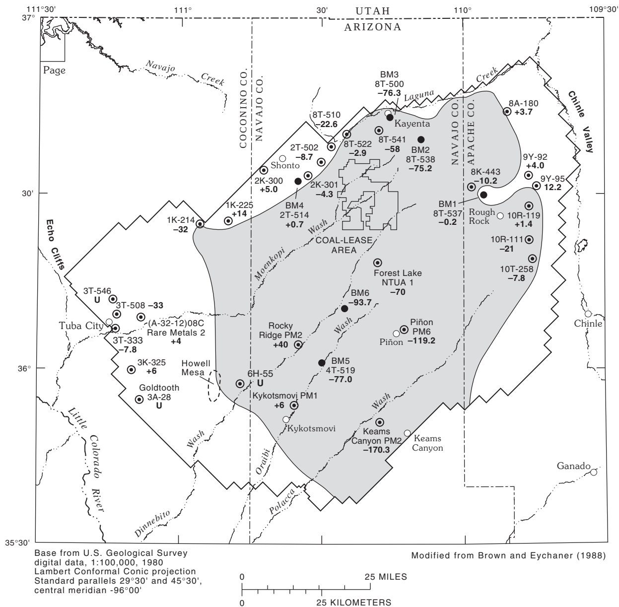
Figure 5. Water-level changes in wells completed in the N aquifer from the prestress period to 1998, Black Mesa, Arizona. See table 4 .
