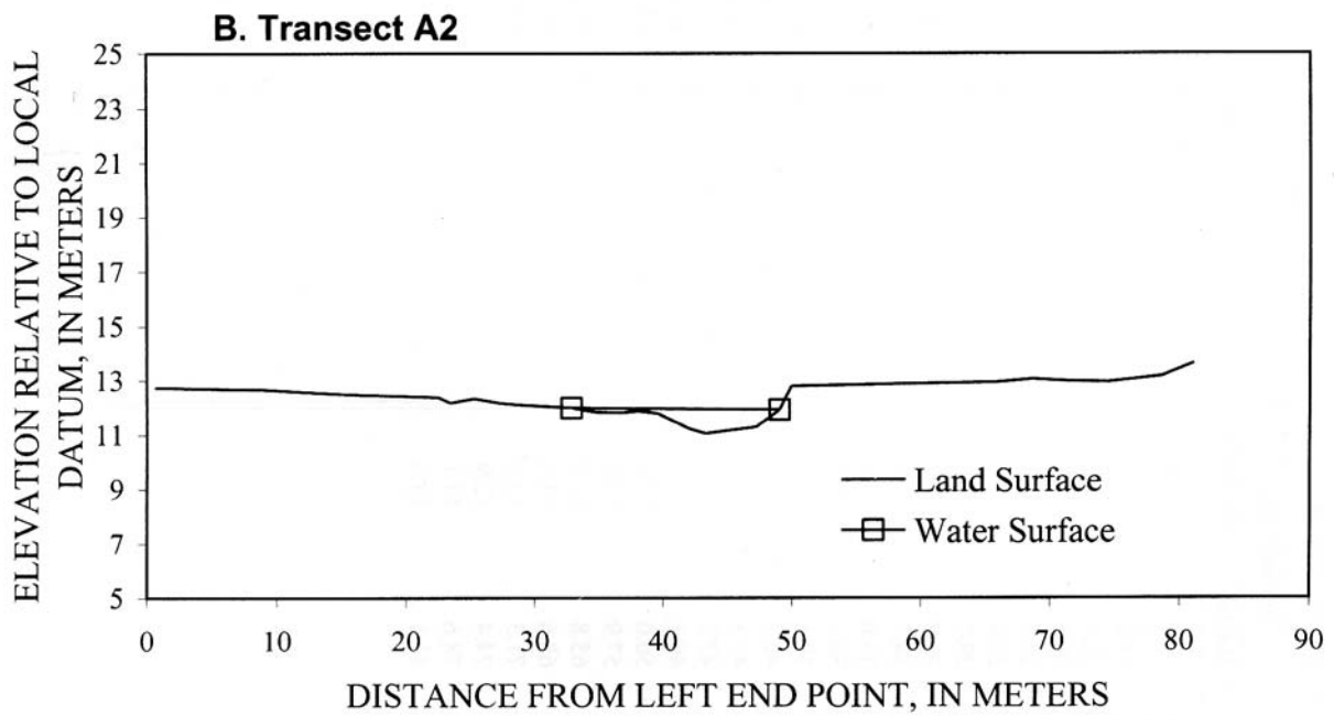
Figure 46A–F. Cross sections of channel, reach A, Salt River near Roosevelt, Arizona, July 27 and 28, 1998. A , Transect A1. B , Transect A2. C , Transect A3. D , Transect A4. E , Transect A5. F , Transect A6. Local datum established using arbitrary elevation.
