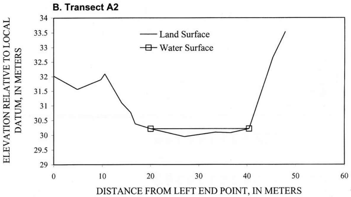
Figure 31 A–F. Cross sections of channel, reach A, Gila River at Kelvin, Arizona, November 3 and 4, 1998. A , Transect A1. B , Transect A2. C , Transect A3. D , Transect A4. E , Transect A5. F , Transect A6. Local datum is the zero point of the reference gage at streamflow-gaging station, Gila River at Kelvin, Arizona (09474000).
