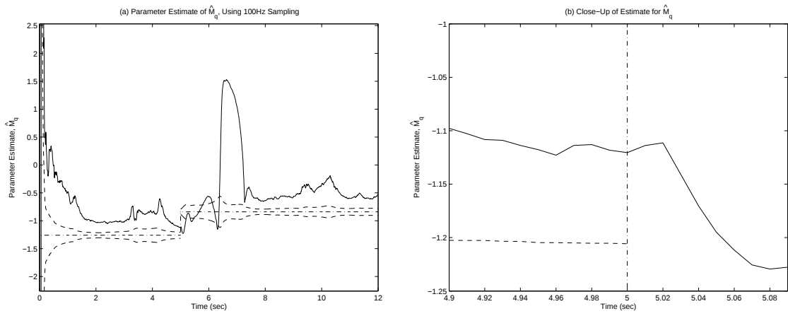
Figure I.4: Estimate of control derivative \hat{M}_q using sliding window batch process. 50% of the horizontal stabilator surface is lost at t = 5\text{s} , but there is not trim change. Sliding window is not reset after failure. Solid lines—estimates, Dash-dot lines—true parameter value about which the 1- \sigma bounds from the filter-predicted equation error covariance (dashed lines) are depicted.
