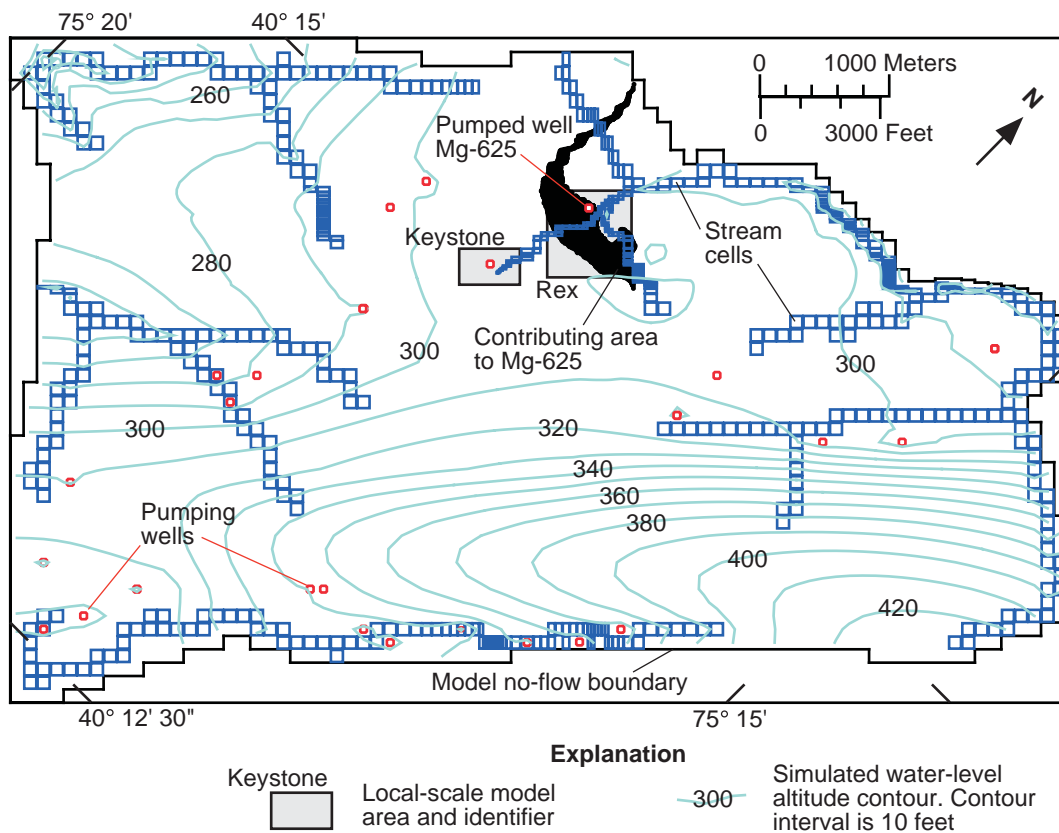
Figure 27. -- Simulated water levels in the upper part of the bedrock aquifer in Lansdale, Pa., and vicinity for 1997 conditions and contributing area for well Mg-625 pumping at a rate of 30 gallons per minute.
