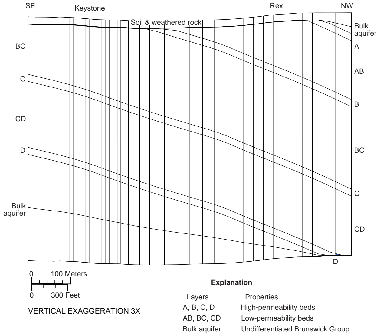
Figure 24. -- Hydrogeologic cross-section in the downdip direction in northwestern Lansdale. Assumed high-permeability beds are designated A-D. Assumed structural contours of the top of bed A are shown in figure 23.
