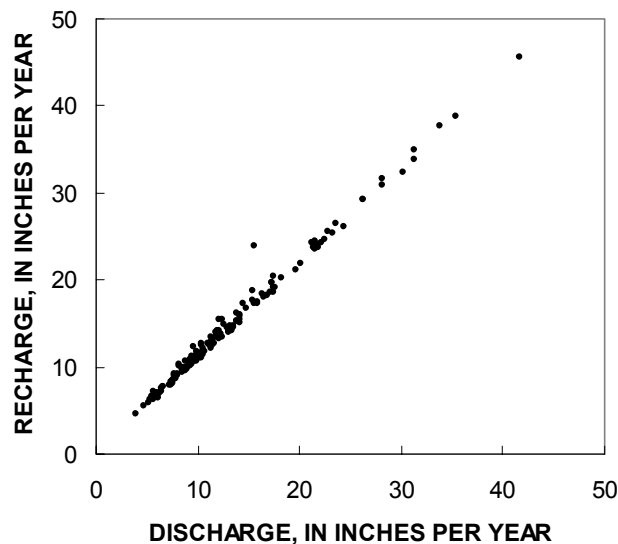
Figure 21. Relation between recharge estimates from the RORA program and discharge estimates from the PART program, on the basis of a large time scale. (Each point represents one of 157 streamflow stations in the AP-RASA project and gives the mean for the time period 1981-90.).
