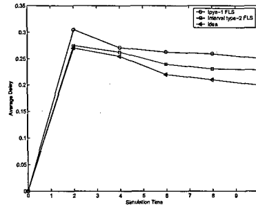
Figure 6: Average Delay for Three Algorithms
