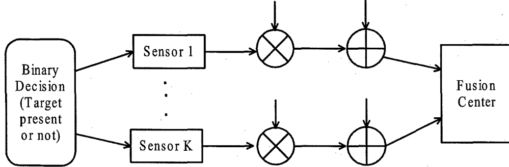
Figure 2: Single-target, single-hop decision fusion model
