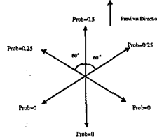
Figure 1: One-step Markov Path Model
