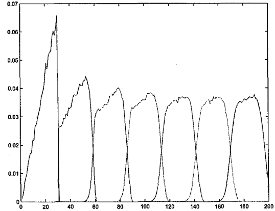
Fig. 5. Histograms of hop-distance joint distribution. ( R = 30 , \lambda = 6.37(10)^{-3} )
