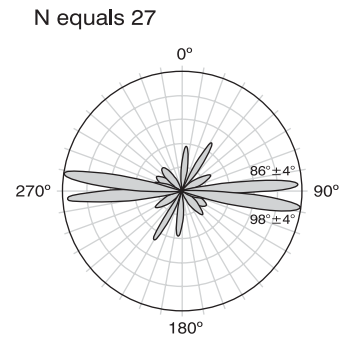
Figure 4. Contoured stereo-net plots and azimuth-frequency plots showing fracture data for (A) all fractures, (B) Exeter Diorite, (C) Kittery Formation, (D) Eliot Formation, (E) diabase dikes and sills, and (F) open and vug-filled fractures at Great Bay, N.H. N equals the number of fracture data measurements represented. The length of the family peaks on the azimuth-frequency plots indicates the normalized height. Principal peaks with normalized concentrations greater than 50 percent are labeled. Circle interval equals 20 percent, increasing outward.
