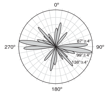
Figure 5. Contoured stereo-net plots and azimuth-frequency plots showing fracture data binned by spacing for (A) 1- to 4-centimeter spacing, (B) 5- to 10-centimeter spacing, (C) 11- to 40-centimeter spacing, and (D) 41- to 200-centimeter spacing at Great Bay, N.H. N equals the number of fracture data measurements represented. The length of the family peaks on the azimuth-frequency plots indicates the normalized height. Principal peaks with normalized concentrations greater than 50 percent are labeled. Circle interval equals 20 percent, increasing outward.
