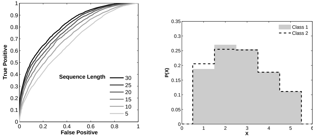
Figure 20. ROC curves for various sequence length settings. Discrete probability distribution for the 2 class problem.
