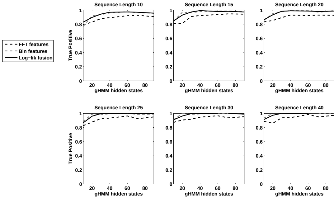
Figure 39. Fusion of multi-dimensional Gaussian HMMs using mean log-likelihoods. Prior knowledge of target aspect angle as a function of the number of hidden states is used.
