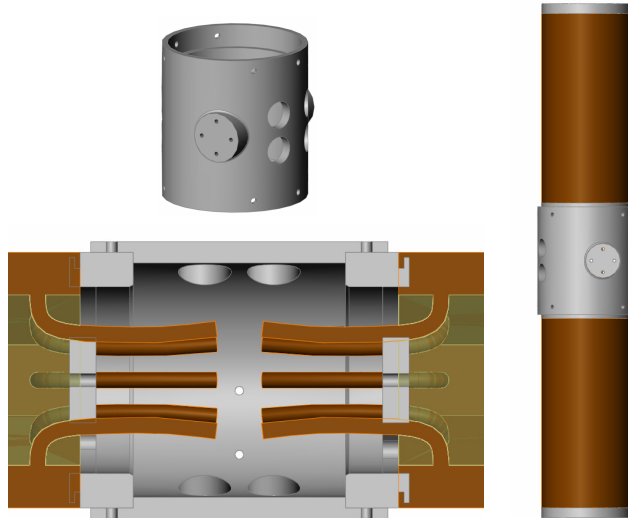
Figure 12 – Source Array Center Mounting
