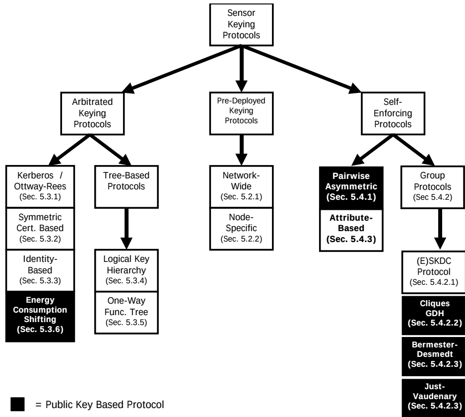
Figure 8 - SAFEMITS Network Keying Protocols
