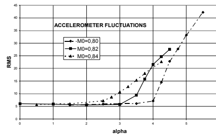
Figure 18 – Buffeting onset for each tested flow Mach number.
