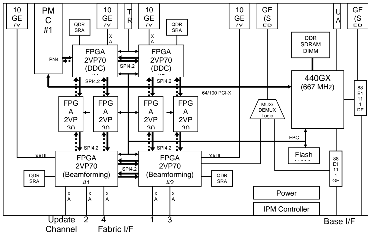
Figure 4: DDM Build 3 Board Configuration
