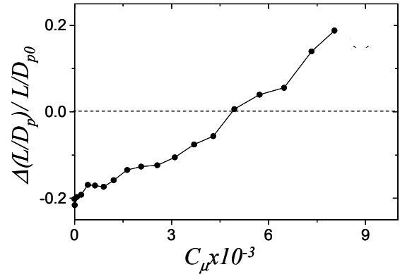
Figure 14 Variation with C_\mu of the normalized increments of the lift to drag ratio for \alpha = 0^\circ .
