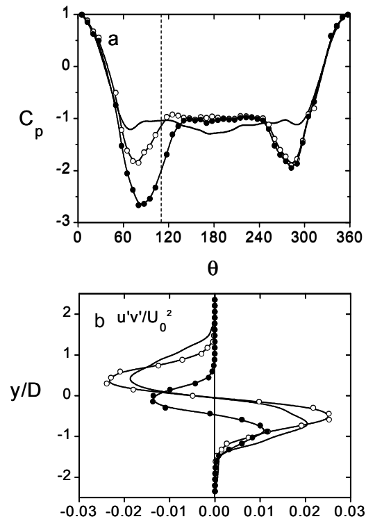
Figure 6. Azimuthal pressure distribution (a) and Reynolds stress (b) with boundary layer trip: unforced (○), forced (●), baseline (—).
