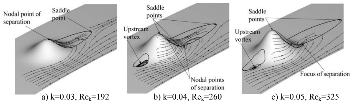
Figure 6. Shear topological change for increasing roughness height.
