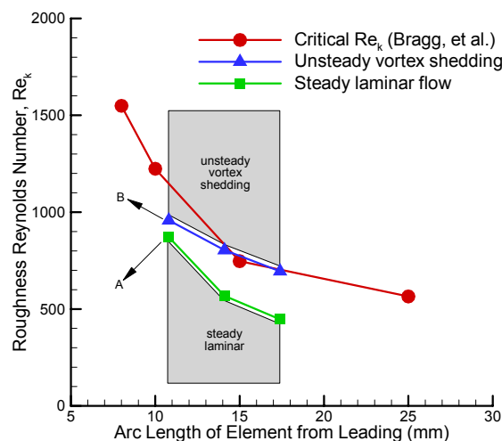
Figure 3. Comparison of steady laminar and unsteady vortex-shedding flow past roughness element to critical roughness Reynolds number.
