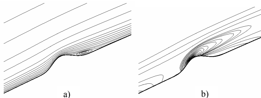
Figure 2. Laminar flow past single leading-edge hump: a) stream function contours and b) vorticity contours.
