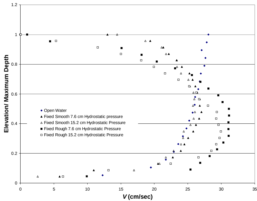
Figure 6. Velocity profiles for open water and fixed smooth and rough ice covers with hydrostatic heads of 7.6 and 15.2 cm. V_{avg} = 23.56 \text{ cm/s} , V_{avg}/V_c = 0.8589 .
