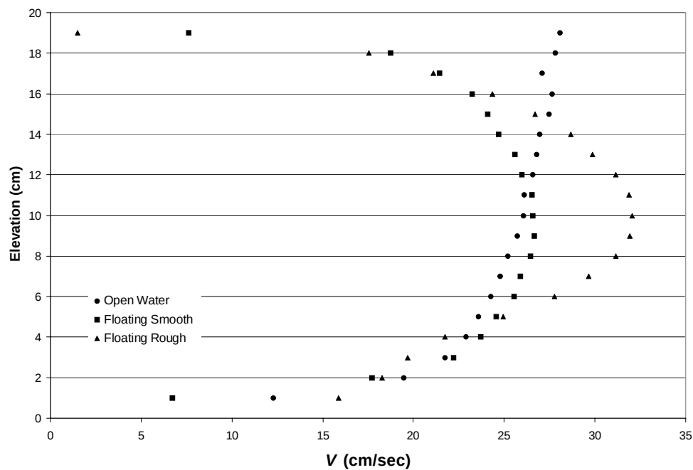
Figure 5. Velocity profiles for open water and floating smooth and rough ice covers. V_{avg} = 23.56 \text{ cm/s} , V_{avg}/V_c = 0.8589 .
