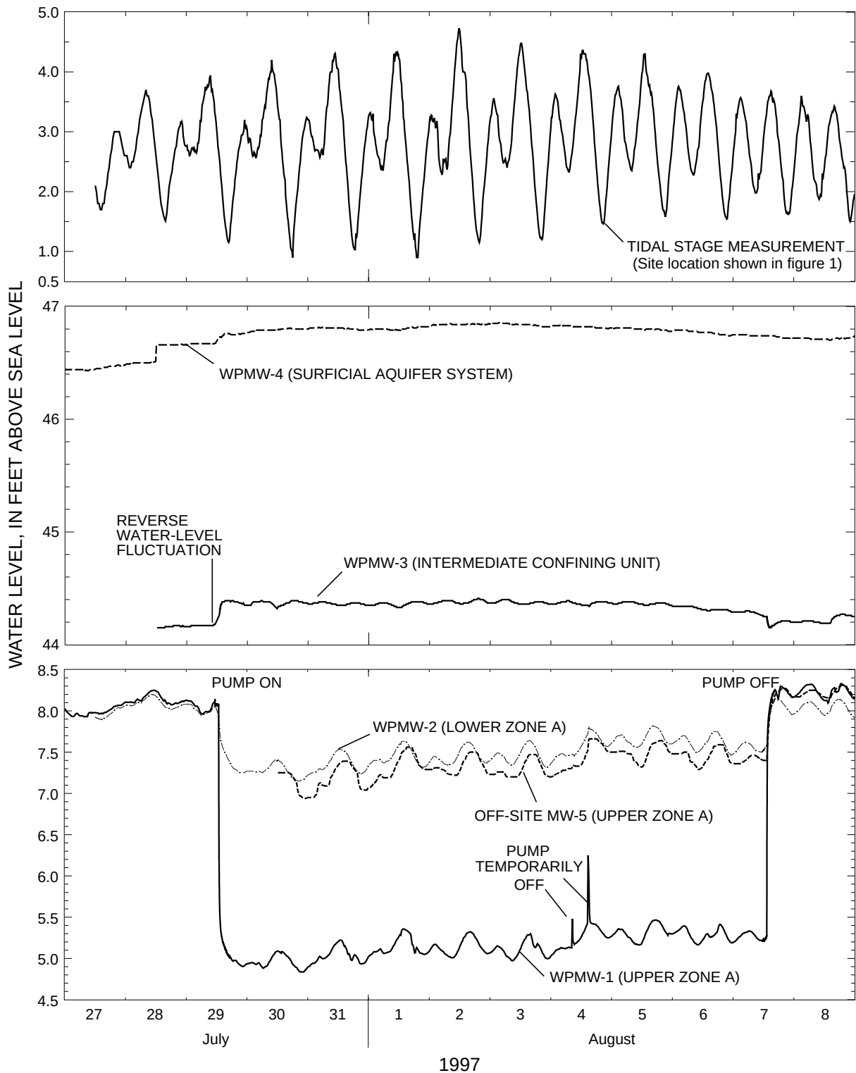
Figure 9. Water levels in all monitor wells before, during, and after the 9-day aquifer test.
