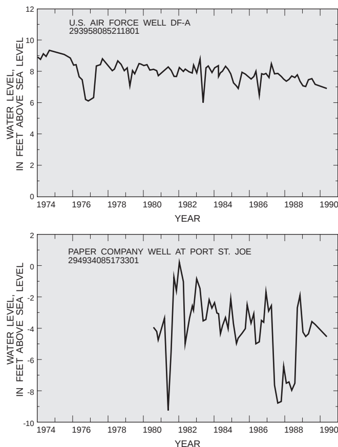
Figure 2. Hydrographs for two wells near St. Joseph Bay, 1974-90.
