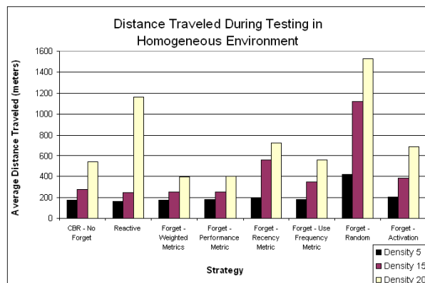
Fig. 5. This graph shows the distance traveled by the robots during the missions. Three obstacle densities were tested for the homogeneous maps. Notice the performance and weighted metrics outperformed both the purely reactive system as well as the original CBR architecture for higher densities.
