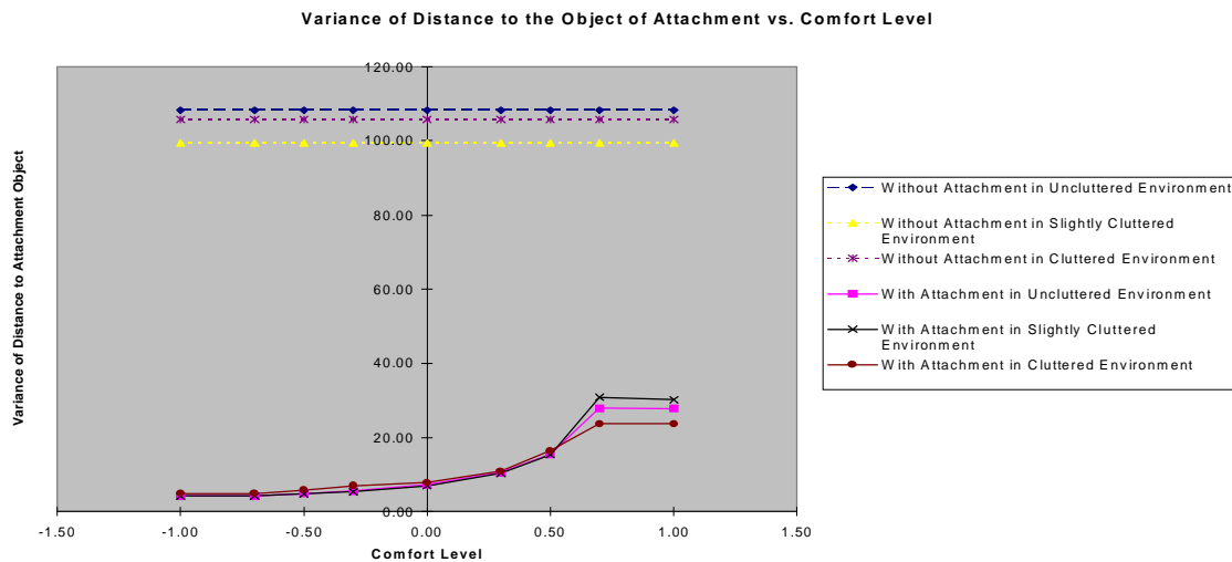
Figure 6. The variance of the distance from the robot to its object of attachment without the attachment behavior (top horizontal lines) and with the attachment behavior enabled (bottom non-linear curves) in obstacle-free, slightly cluttered and significantly cluttered environments.
