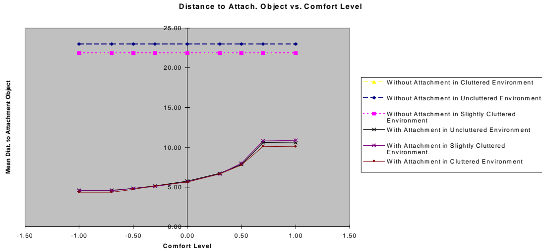
Figure 5. The average distance from the robot to its object of attachment without the attachment behavior (top horizontal lines) and with the attachment behavior enabled (bottom non-linear curves) in obstacle-free, slightly cluttered and significantly cluttered environments.
