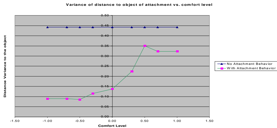
Figure 10. The variance of the distance from the robot to its object of attachment without the attachment behavior (top horizontal line) and with the attachment behavior enabled (bottom non-linear curve) for real-robot experiments.
