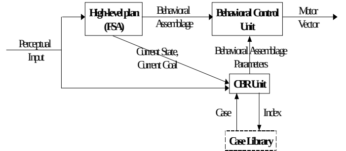
Figure 2. Integration of the case-base reasoning unit within the AuRA architecture.
