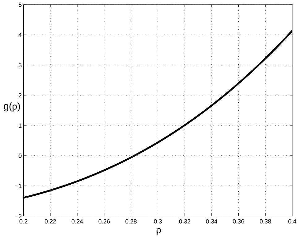
Fig. 4.1.5. Plot of \rho versus g(\rho) , where g is given by the left hand side of (78)
