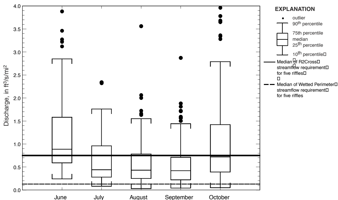
Figure 10. Distribution of mean monthly discharges for the period 1969-1998 for streamgaging stations 01096000, 01097300, 01105600, 01111500, and 01175670 compared with median streamflow requirements estimated by the R2Cross and Wetted-Perimeter methods for five riffles in the Assabet and Charles River Basins, Massachusetts.
