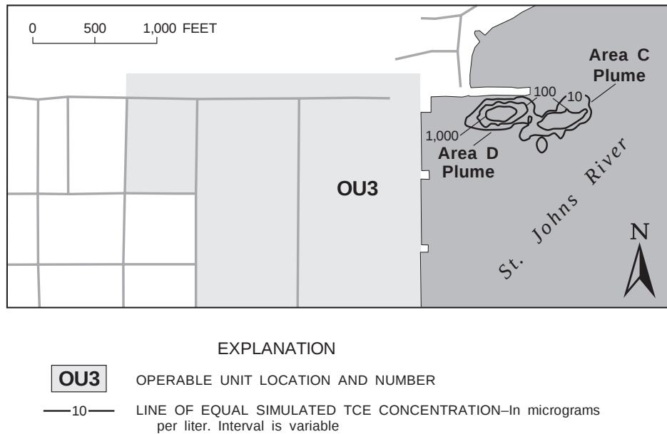
Figure 32. Simulated trichloroethene (TCE) concentrations in layer 1 after 100 years traveltime and assuming average dispersion.
