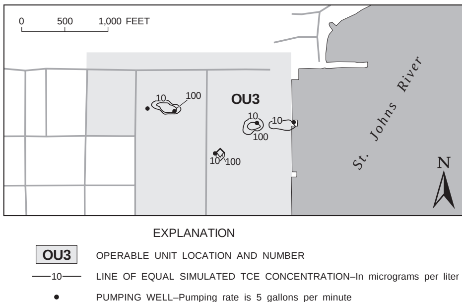
Figure 34. Simulated trichloroethene (TCE) concentrations in layer 3 after 10 years of pumping.
