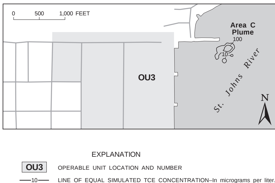
Figure 24. Simulated trichloroethene (TCE) concentrations in layer 1 after 60 years traveltime and assuming relatively low dispersion.
