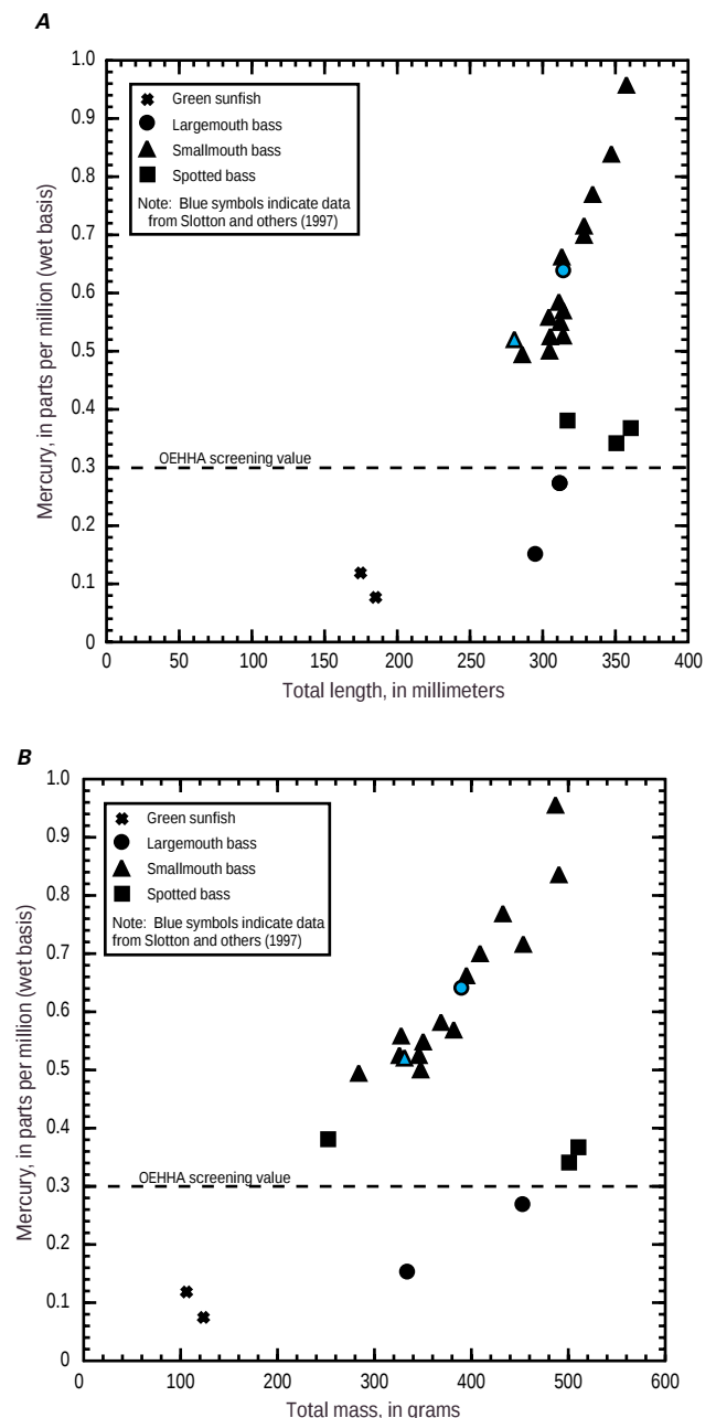
Figure 4. Mercury concentration for fish collected from Lake Englebright, California, 1999. A, In relation to total length. B, In relation to total mass. Dashed horizontal line at mercury concentration of 0.3 ppm represents a screening value provided by the Office of Environmental Health Hazard Assessment (Brodberg and Pollock, 1999). Blue symbols indicate data from Slotton and others (1997).
