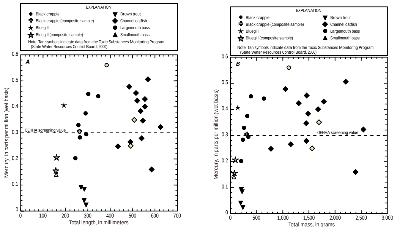
Figure 6. Mercury concentration for fish collected from Rollins Reservoir, California, 1999. A, In relation to total length. B, In relation to total mass. Dashed horizontal line at mercury concentration of 0.3 ppm represents a screening value provided by the Office of Environmental Health Hazard Assessment (Brodberg and Pollock, 1999). Tan symbols indicate data from the State of California's Toxic Substances Monitoring Program (State Water Resources Control Board, 2000); green symbols indicate composite samples from this study.
