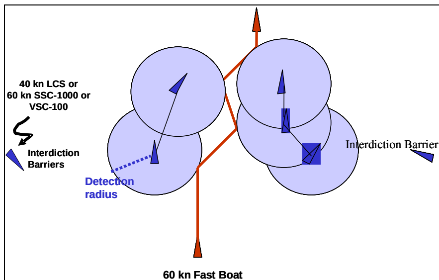
Figure 22. Interdiction Concept
