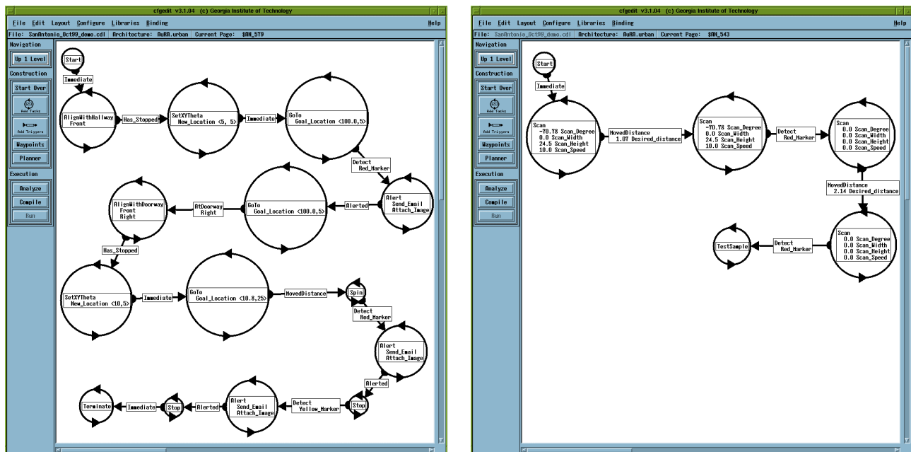
Figure 5: The Finite State Acceptor (FSA) representation of the indoor assessment mission (Phase II): the motor FSA (left) and the camera FSA (right).
