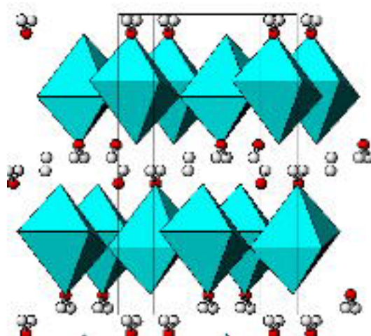
Figure 6 : Projection of the \text{MoO}_3\text{x1H}_2\text{O} structure in the [001] direction.
