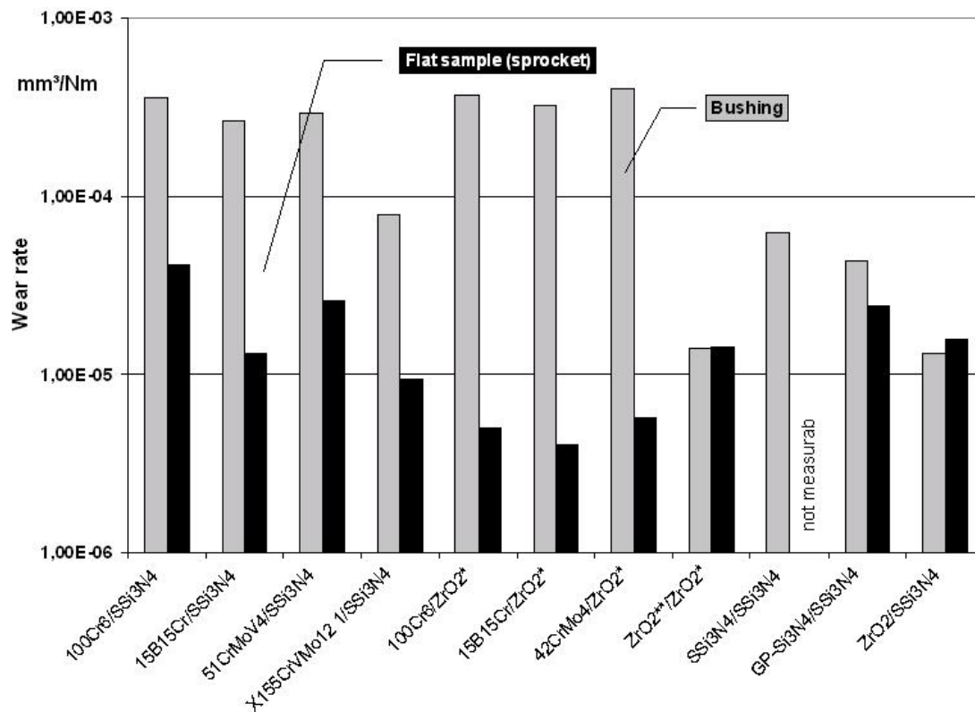
Figure 11 : Comparison the abrasive wear rates \text{Si}_3\text{N}_4 and \text{ZrO}_2 sprockets against steel bushings
