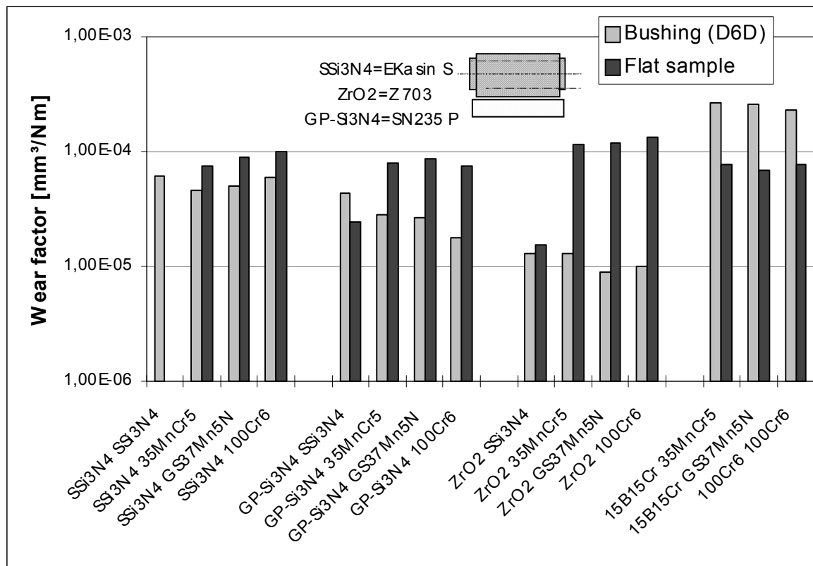
Figure 10 : Comparison the abrasive wear [16] rates of steels, Si 3 N 4 and ZrO 2
