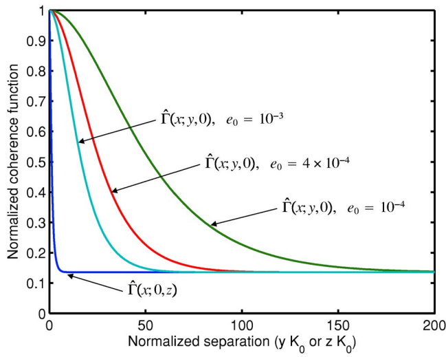
FIG. 6. (Color online) The normalized coherence function \hat{\Gamma}(x; y, z) of a plane sound wave propagating through IGW. The curves show this function for x = \gamma^{-1} and for either a vertical separation ( y=0 ) or a horizontal separation ( z=0 ) between two points of observation. The abscissa is yK_0 for horizontal separations or zK_0 for vertical separations. Three curves are shown for horizontal separations, which correspond to e_0 = 10^{-4} , e_0 = 4 \times 10^{-4} , and e_0 = 10^{-3} .
