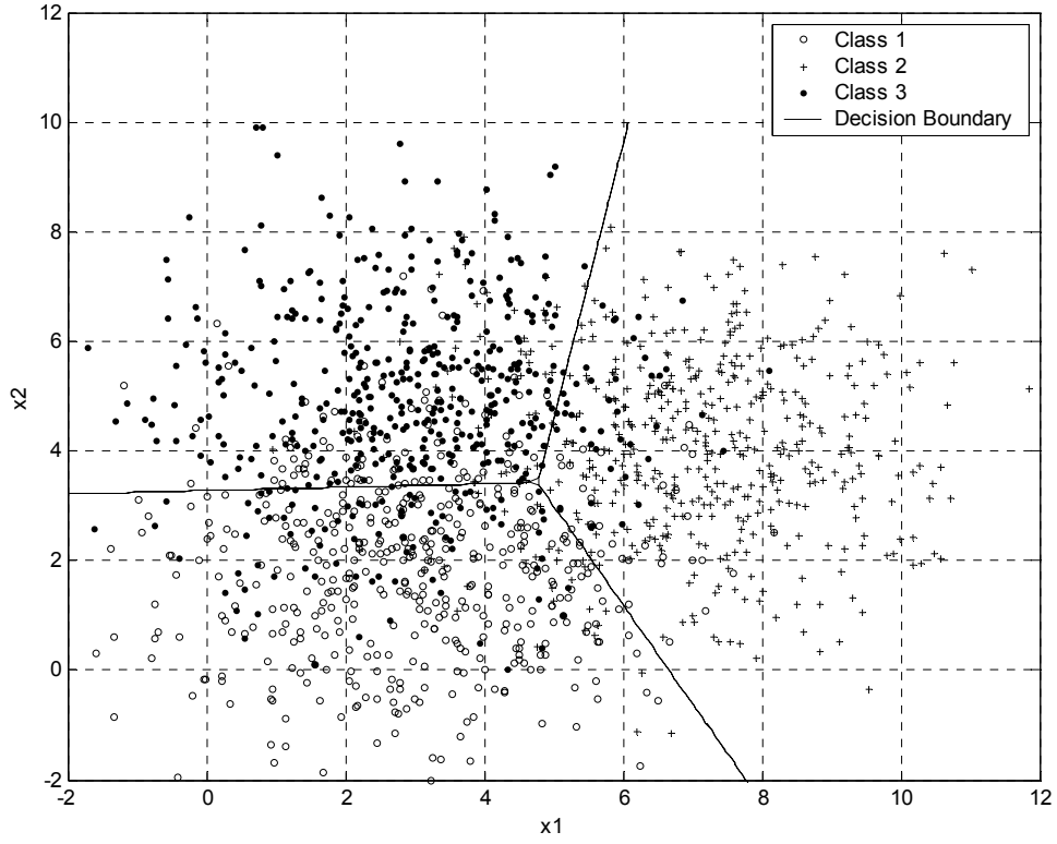
Figure 12. Randomly generated data in three classes are separated by linear decision boundaries. The class means are \mu_1 = [3 \ 2]^T , \mu_2 = [7 \ 4]^T , \mu_3 = [3 \ 5]^T and have equal across class covariance matrices, \Sigma_1 = \Sigma_2 = \Sigma_3 = \begin{bmatrix} 3 & 0 \\ 0 & 3 \end{bmatrix} .
