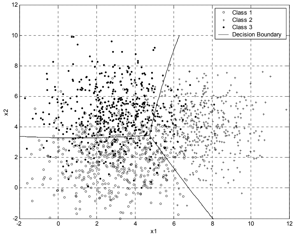
Figure 16. Randomly generated data consisting of three classes are separated by a linear decision boundary produced by quadratic discriminant analysis. The class means are \mu_1 = [3 \ 2]^T , \mu_2 = [7 \ 4]^T , \mu_3 = [3 \ 5]^T and have equal across class covariance matrices, \Sigma_1 = \Sigma_2 = \Sigma_3 = \begin{bmatrix} 3 & 0 \\ 0 & 3 \end{bmatrix} .
