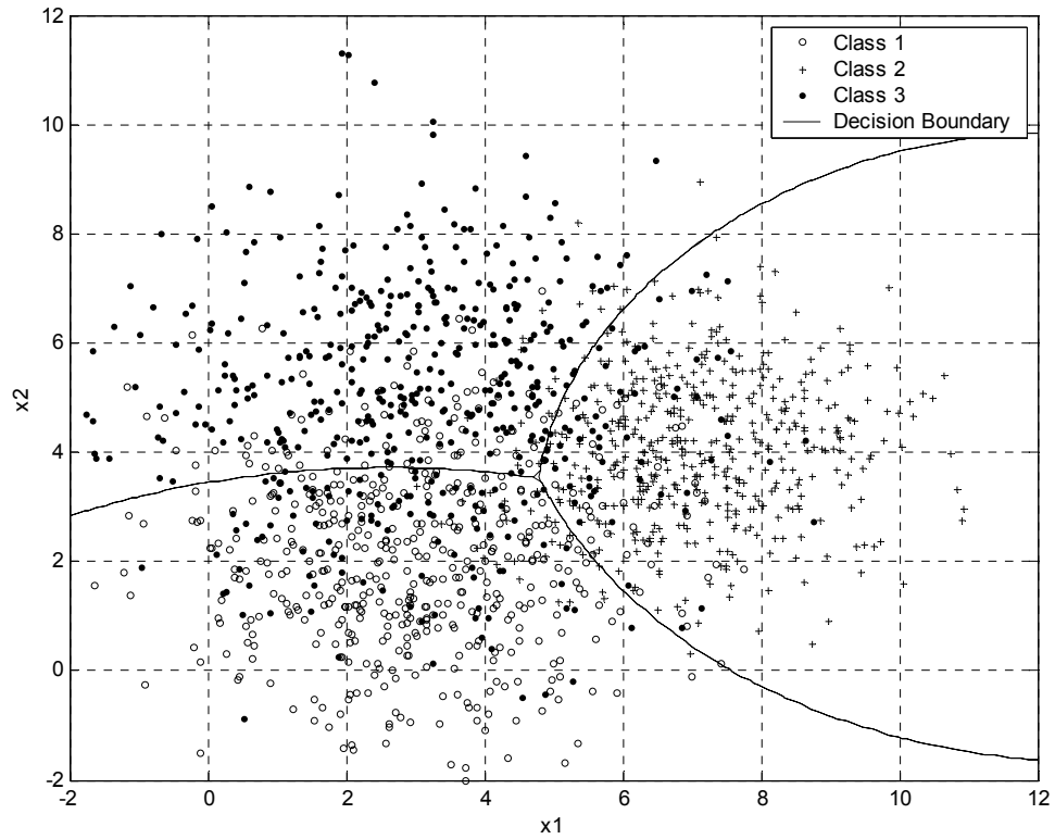
Figure 17. Randomly generated data consisting of three classes are separated by curvilinear decision boundaries produced by quadratic discriminant analysis. The class means are \mu_1 = [3 \ 2]^T , \mu_2 = [7 \ 4]^T , \mu_3 = [3 \ 5]^T and have unequal across class covariance matrices, \Sigma_1 = \begin{bmatrix} 3 & 0 \\ 0 & 3 \end{bmatrix} , \Sigma_2 = \begin{bmatrix} 2 & 0 \\ 0 & 2 \end{bmatrix} , \Sigma_3 = \begin{bmatrix} 4 & 0 \\ 0 & 4 \end{bmatrix} .
