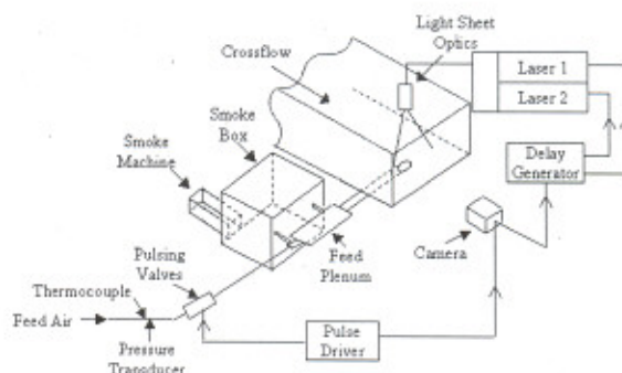
Figure 2. Schematic of PIV setup
