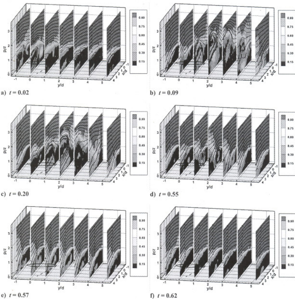
Figure 6. Normalized velocity plots (velocity magnitude divided by U_\infty ) for B = 2 , F^+ = 0.004 , \Delta = 50\% case
