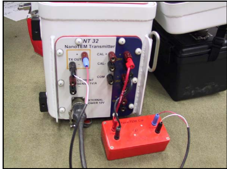
Figure 3.7: Photograph showing passive NT Calibrator circuit connected to the NT-32 II transceiver.
