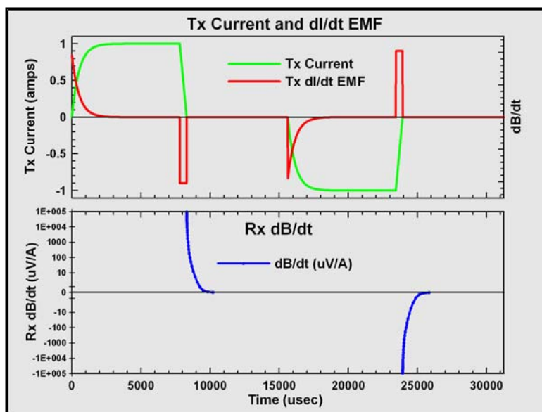
Figure 2.1: Schematic illustration of a TEM transmitter current waveform (green curve), the EMF induced in the target (red), and the resulting secondary magnetic field measured at the receiver loop (blue).
