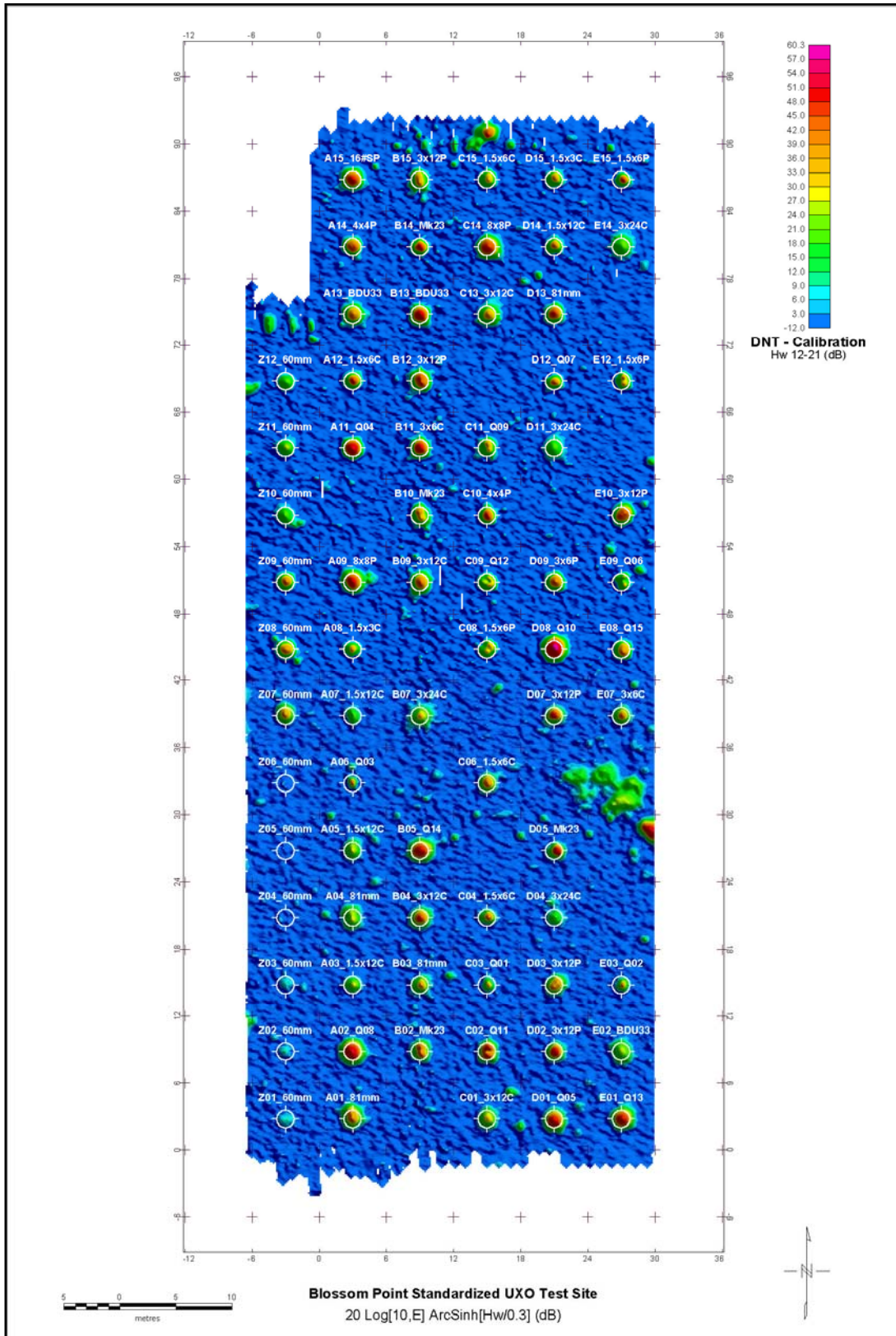
Figure 2.18: Map of compounded vertical dBw/dt field for an intermediate composite time gate over Blossom Point.
