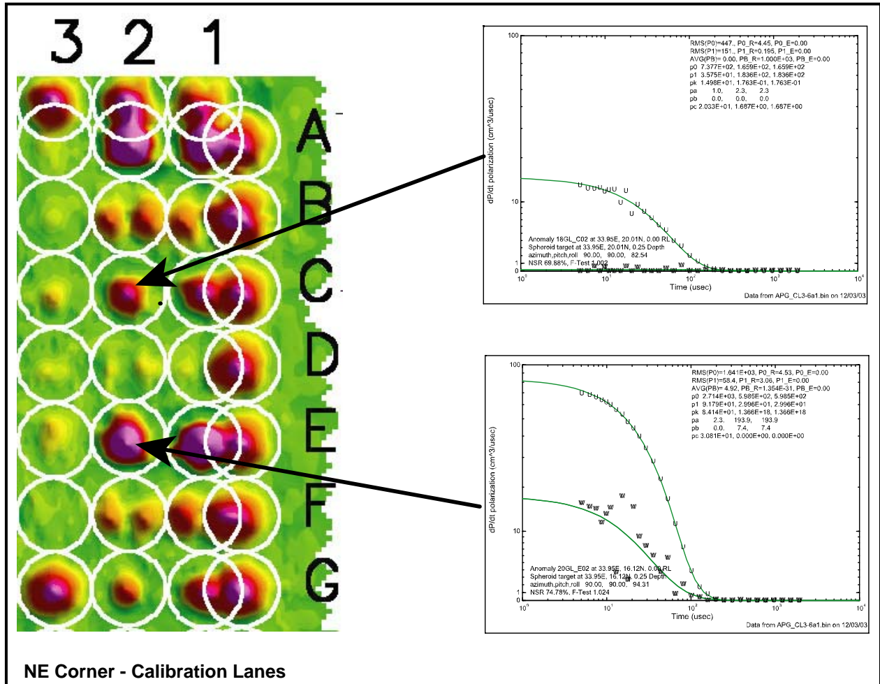
Figure 4.3: Polarizability plots for clutter-masked 60mm targets at the Calibration Lanes of the Standardized Test Site at ATC.
