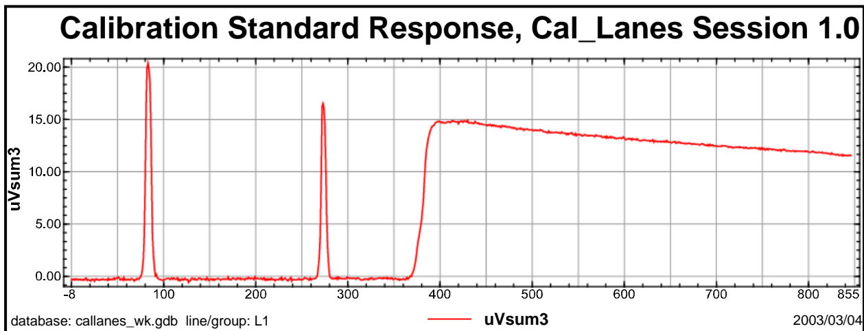
Figure 3.11. An example of unstable system response in DNT data from a calibration run made without sufficient system warm-up time. Uvsum3 is the vertical component, dBz/dt, composite windows 12-21.
