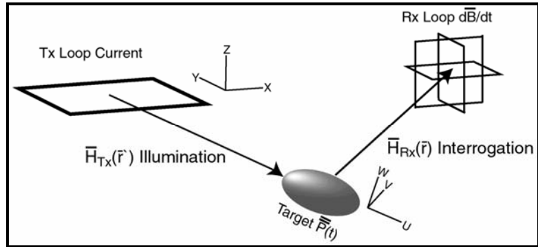
Figure 2.17: Schematic of anisotropic point-dipole model.
