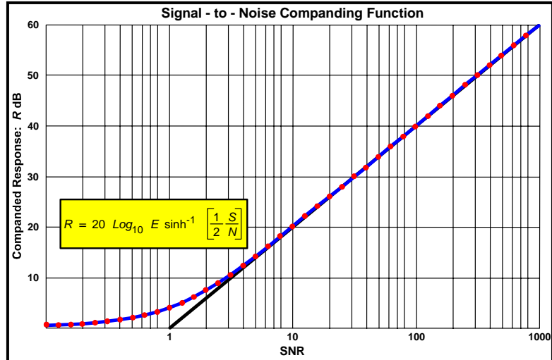
Figure 3.15: Function used to affect bipolar companding. When scaled as indicated in the formula, the function approximates the signal-to-noise ratio (SNR) expressed in dB for SNR>1.
