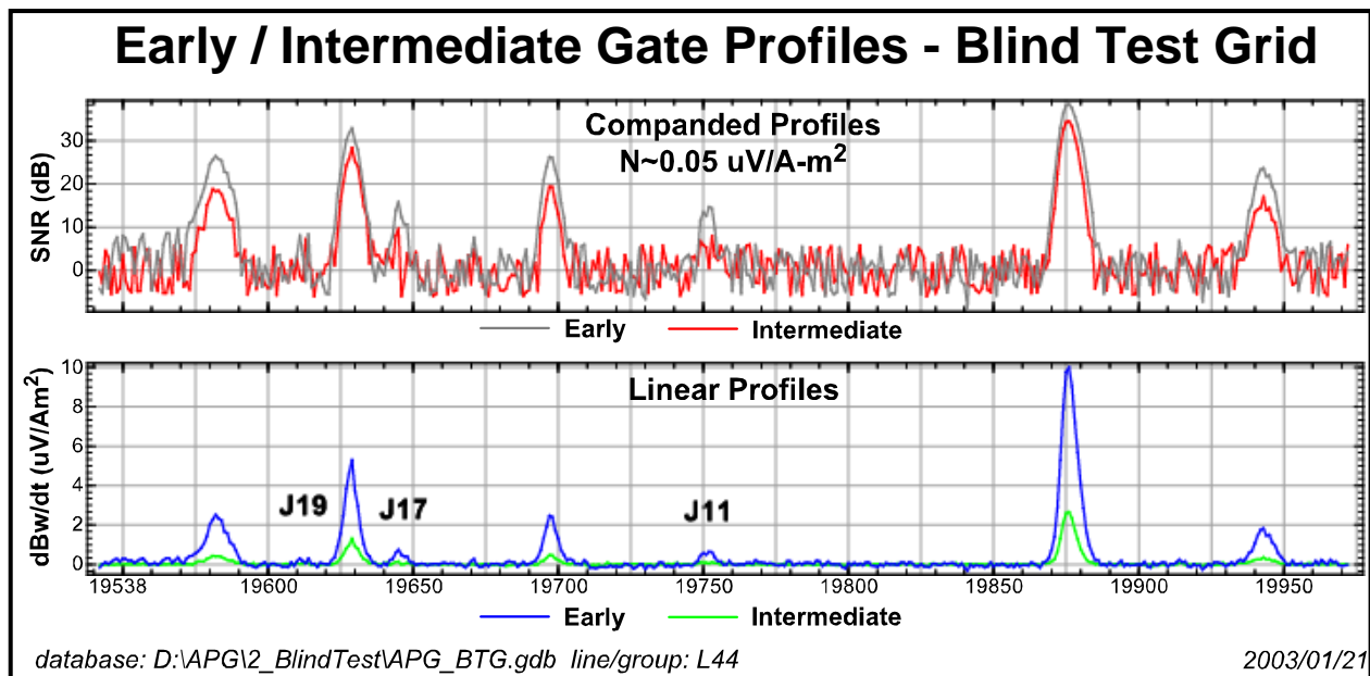
Figure 3.16: DNT profiles at Early (10 \mu s ) and Intermediate (68 \mu s ) time composite gates illustrate improved SNR at early times.
