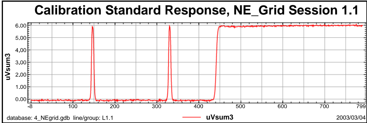
Figure 3.10. An example calibration run standard response plot for the vertical component, dBz/dt, composite windows 12-21 (uVsum3).
