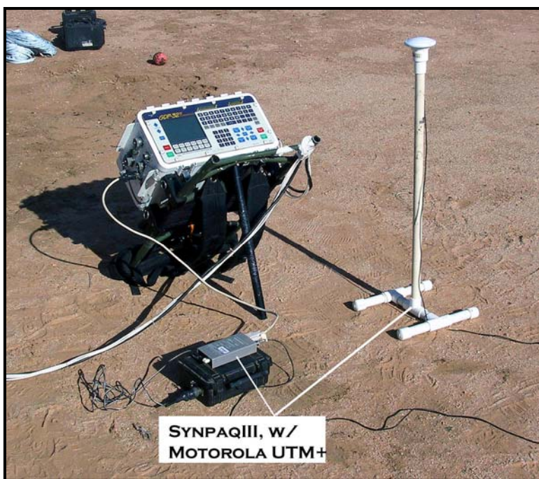
Figure 2.8: Photograph showing setup for time synchronization of the NT-32 II using a SynpaqIII (Synergy Systems, San Diego) with Motorola UTM+ GPS engine.
