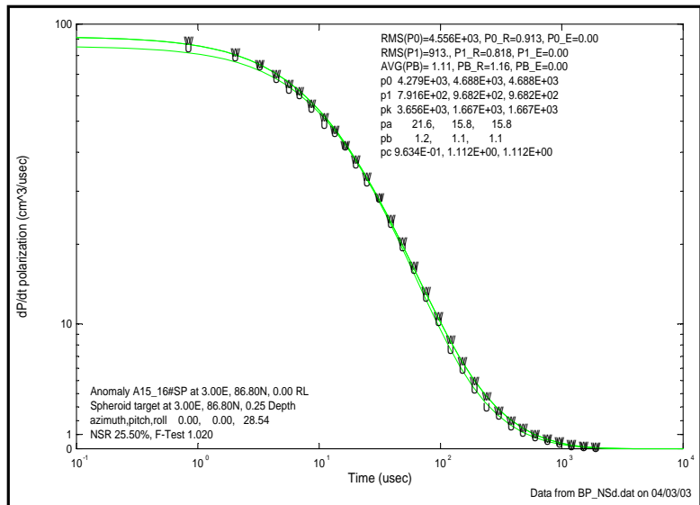
Figure 2.19: Polarizability transients for a 16 lb shotput show the symmetry expected for a spherical object, dP_u/dt = dP_v/dt = dP_w/dt . Pasion model b values > 0.8 indicate a permeable object.
