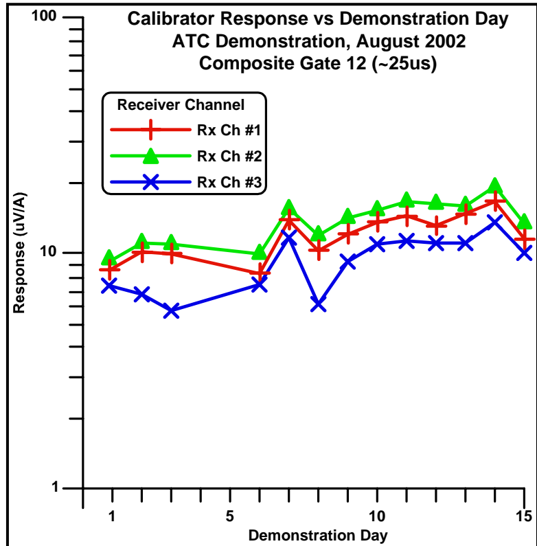
Figure 3.8: Calibrator response as a function of demonstration day for NanoTEM gate 12 (~25 us after current turn-off). The figure shows a systematic difference between the 3-channels in the early time response.
