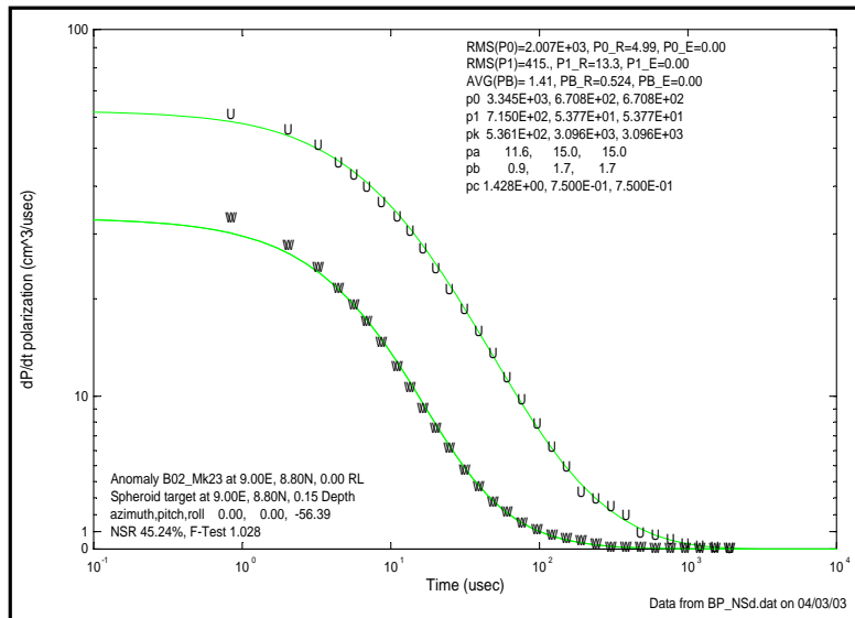
Figure 2.21: Polarizability transients for a Mk23 indicate a ferrous cylindrical object with rod-like symmetry. Pasion model b is greater than 0.8, indicating a permeable object and longitudinal polarizability dPu/dt is greater than two nearly equal transverse polarizability responses, dPv/dt = dPw/dt.
