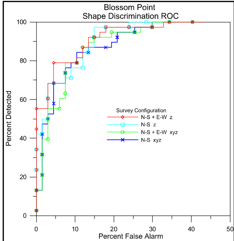
Figure 2.27: Discrimination ROC curves for Blossom Point showing relative performance for single component and multi-component DNT data.
