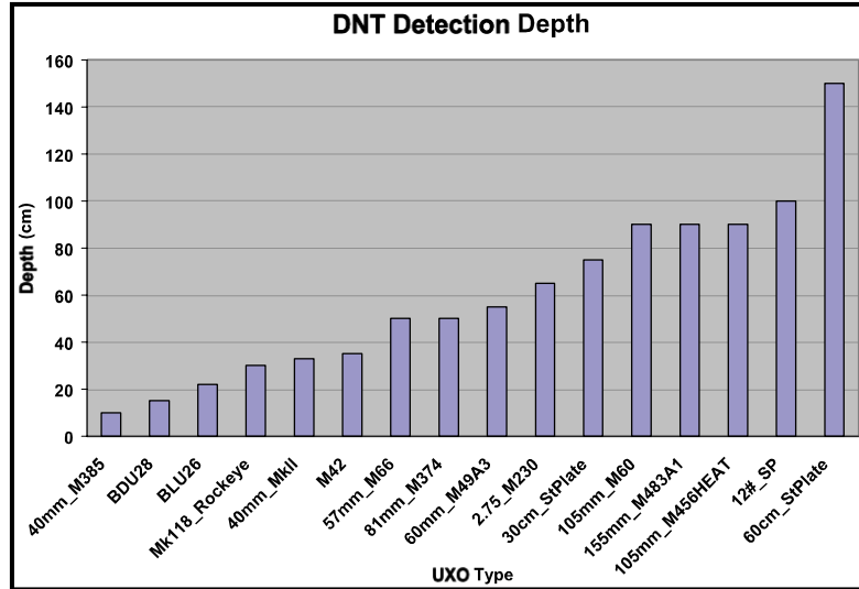
Figure 4.2: Figure summarizing the maximum DNT detection depth for targets in the Calibration Lanes at ATC.
