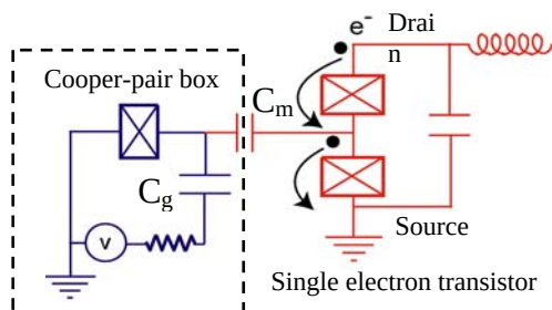
Figure 1: Schematic of Cooper-pair box qubit (CPB) and single electron transistor (SET) readout amplifier. The boxes with crosses denote small-capacitance Josephson junctions. The
