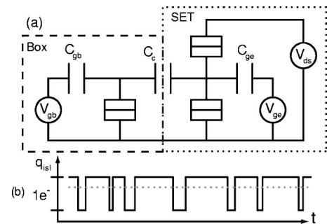
FIG. 1. (a) Circuit diagram of the single-electron box (dashed box) capacitively coupled to the SET (dotted box). The normal-state tunnel junctions are represented by boxes with a single line through them. (b) Plot of the charge state on the SET island vs time. The dotted line shows the mean value of the charge on the SET island.
