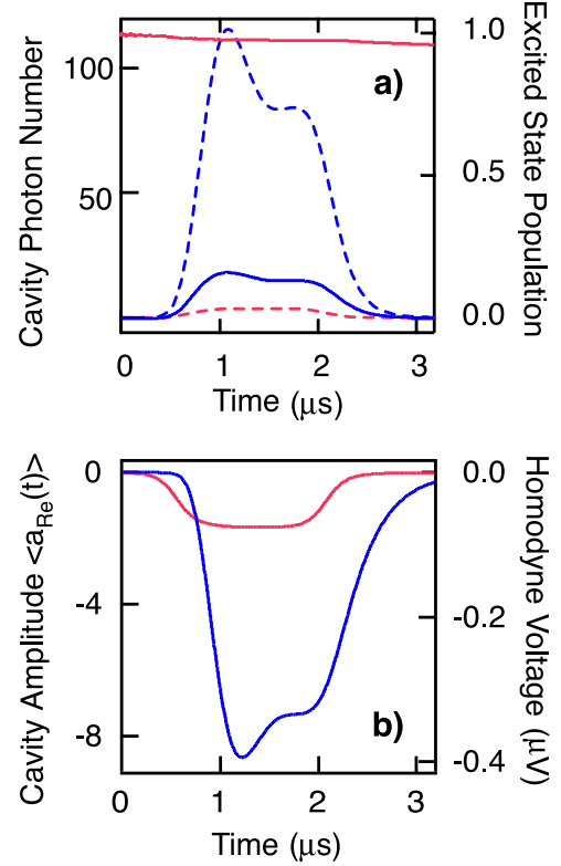
FIG. 6: (color online). Results of numerical simulations using the quantum state diffusion method. A microwave pulse of duration \sim 15/\kappa and centered at the pulled frequency \omega_r + g^2/\Delta drives the cavity. a) The occupation probability of the excited state (right axis, full lines), for the case in which the qubit is initially in the ground (blue) or excited (red) state and intracavity photon number (left axis, dash lines), are shown as a function of time. Though the qubit states are temporarily coherently mixed during the pulse, the probability of real transitions is seen to be small. Depending on the qubit’s state, the pulse is either on or away from the combined cavity-qubit resonance, and therefore is mostly transmitted or mostly reflected. b) The real component of the cavity electric field amplitude (left axis), and the transmitted voltage phasor (right axis) in the output transmission line, for the two possible initial qubit states. The parameters used for the simulation are presented in Table I.
