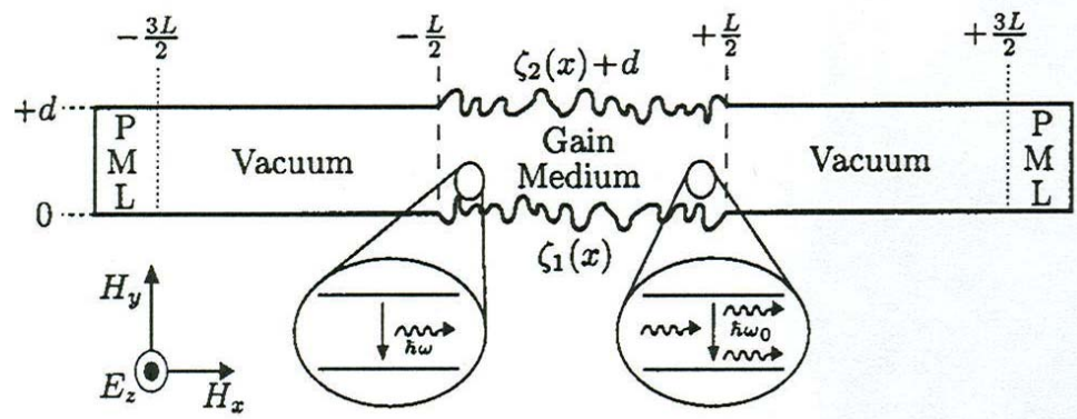
Figure 2.6-1: Layout of the two-dimensional waveguide system.
