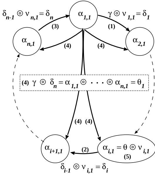
Figure 1. Distributed initialization algorithm
