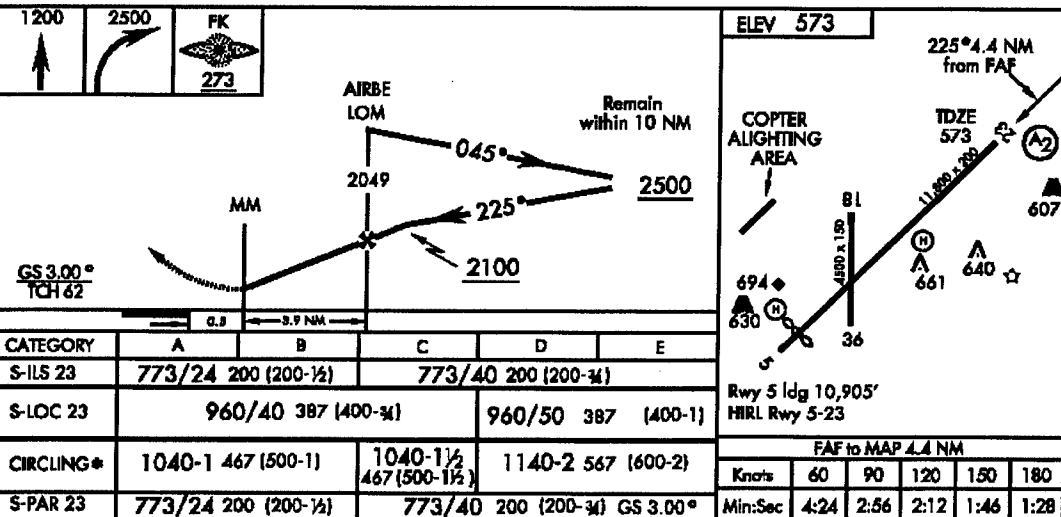
Figure B-2. Campbell Army Airfield ILS RWY 23.
