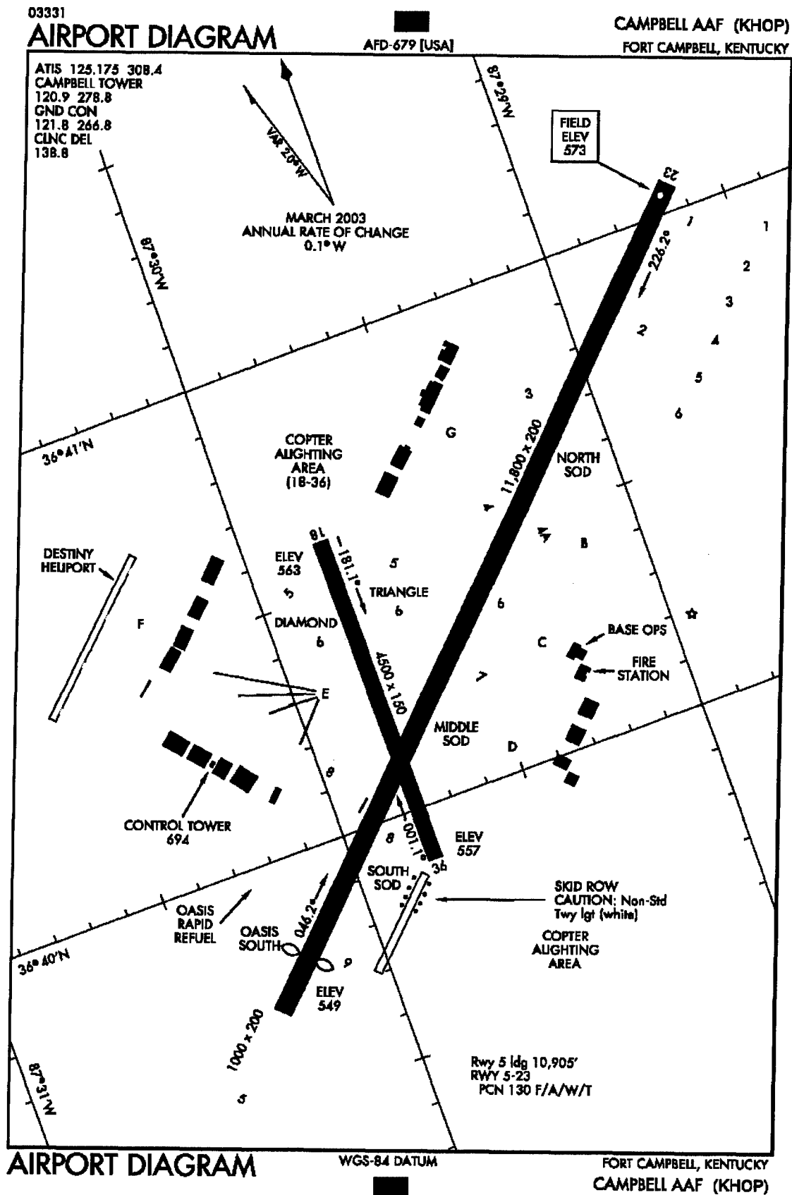
Figure B-1. Campbell Army Airfield airport diagram.
