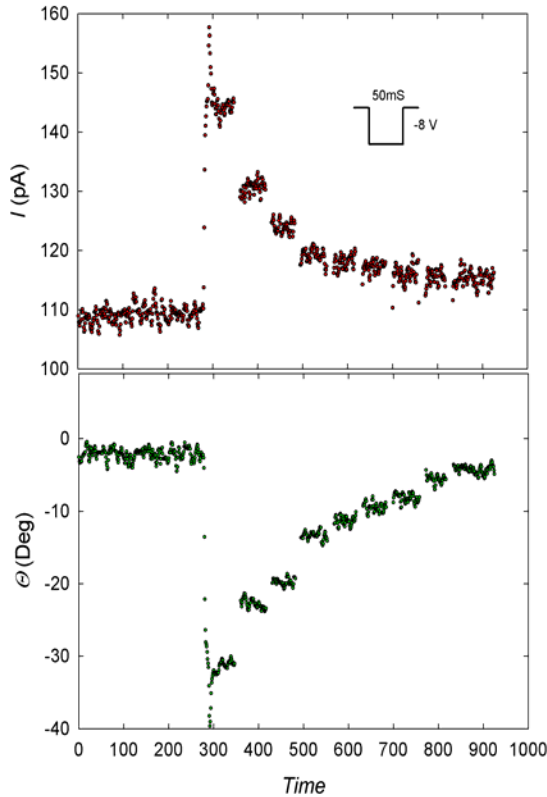
Figure 15. Amplitude and phase of the current through the 2D electron layer on the liquid helium. Each step represents the release of a few hundred electrons trapped on the surface of liquid helium.
