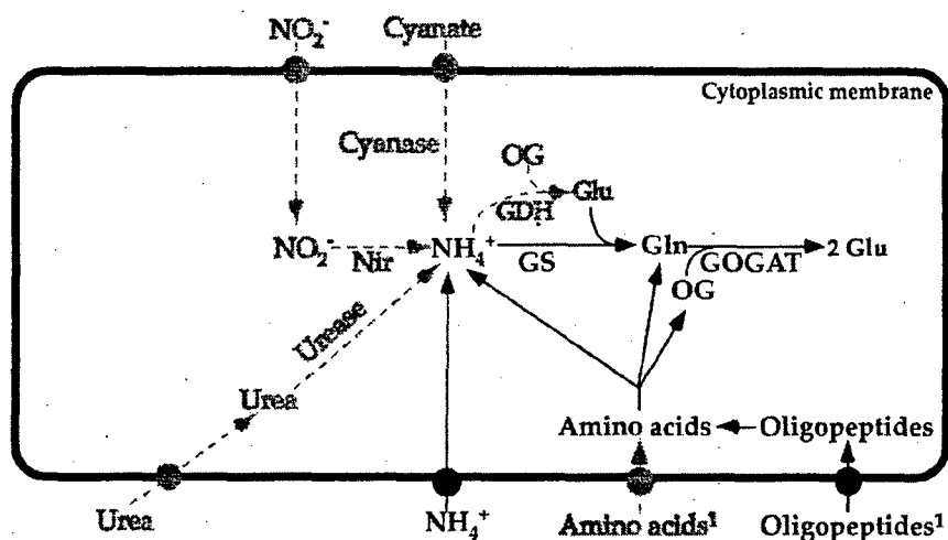
Fig. 6. Diagram of the Prochlorococcus cell showing discrete transport and assimilatory routes used for different N sources. Gray indicates N sources utilized by some, but not all, Prochlorococcus strains. Note that all N sources must first be reduced to ammonia before being assimilated as biomass (Garcia-Fernandez et al., 2004).
