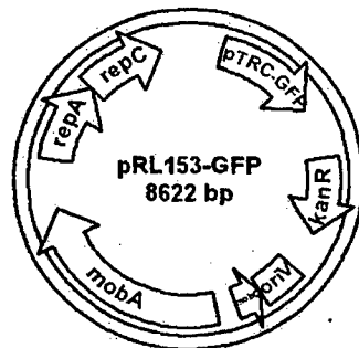
Fig. 9. Replicating plasmid for conjugal transfer to Prochlorococcus . pRL153 is a kanamycin-resistant derivative of the broad host range plasmid RSF1010. It contains an oriT, the requisite mob proteins, and an oriV that replicates in E. coli and diverse cyanobacteria. In addition, it has been modified to express GFP from the synthetic pTRC promoter.
