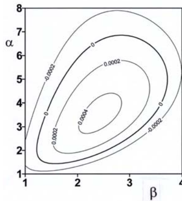
Figure 1. Amplification rates \text{Im}(\sigma) of disturbances in the form of streamwise vortices as a function of the roughness wave number \alpha and the vortex wave number \beta for the flow Reynolds number Re=5000 and the roughness amplitude S=0.0075 .
