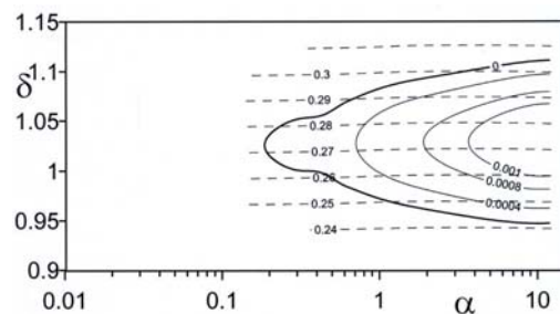
Figure 2. Curves of constant amplification \text{Im}(\sigma) for disturbances in the form of two-dimensional travelling waves for the roughness amplitude S=0.0085 and the flow Reynolds number Re=5600 as a function of the roughness wave number \alpha and the disturbance wave number \delta . Dash lines correspond to \text{Real}(\sigma) .
