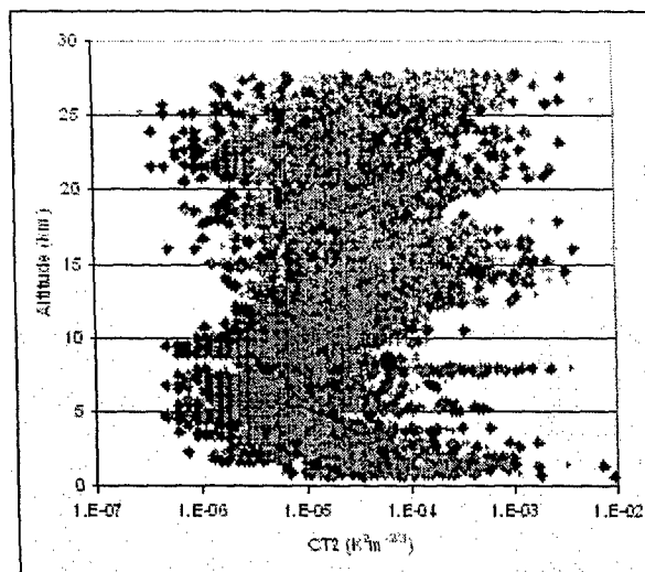
Figure 11. Profiles of C_T^2 from the smaller structure function (small lighter circles) and from the larger (darker diamonds) for flight VOL267.
