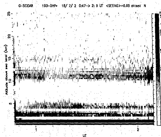
Figure 6. Graphical display of GS results showing a time series of optical turbulence profiles up to 25km above OHP as a function of time for a period from before 1:00 to after 2:00UTC on 18 July 2002. The color scale depicts C_n^2 levels from \sim 1 \times 10^{-18} (white) to 1 \times 10^{-16} \text{ m}^{-2/3} (dark blue).
