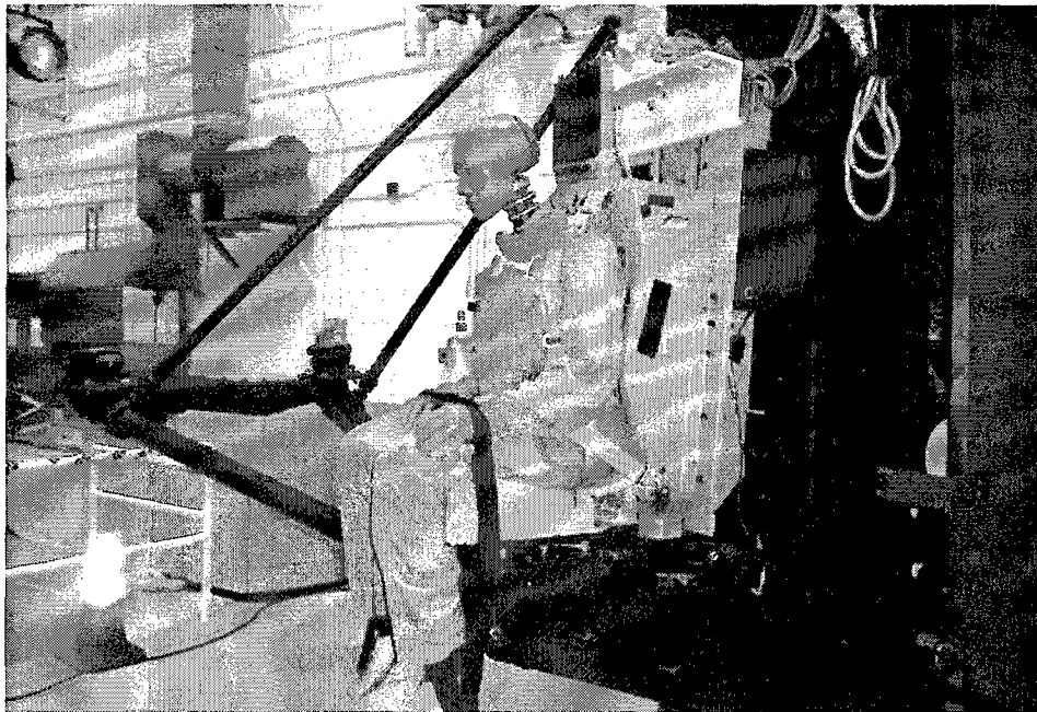
Figure 2: Seat and Manikin
